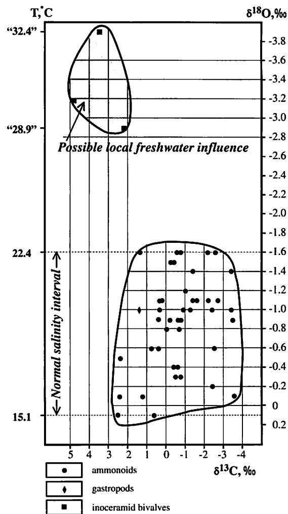
Fig. 11. Plots of \delta^{18}\text{O} and \delta^{13}\text{C} data for aragonitic ammonoid, gastropod and inoceramid bivalve shells from the upper Lower Cenomanian portion of the Mamet Formation, Talovka River Basin.
