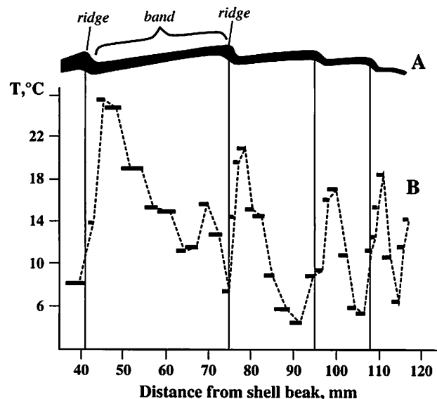
Fig. 2. Recent Swiftopten swifti (Bernardi) shell from Japan sea. A, cross section. B, isotopic temperatures of growth (Zolotarev et al., 1974). Black rectangles and squares indicate the width of the areas along growth striations on shell surfaces from which material was taken for analysis.
