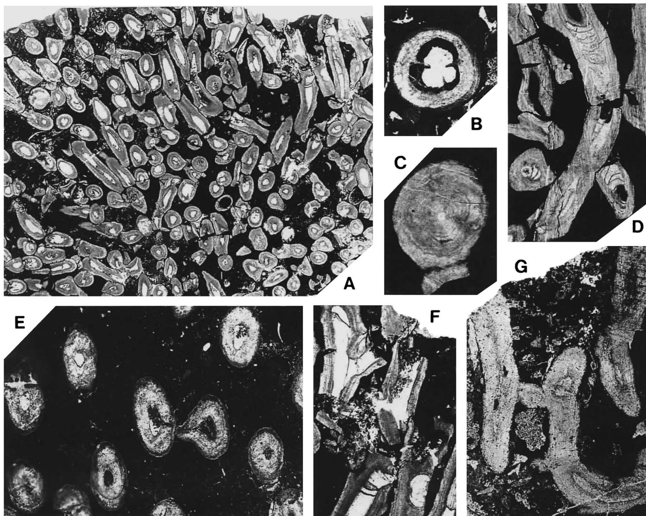
Fig. 7. Multithecopora sp. cf. M. huanglungensis Lee and Chu in Lee et al. , 1930, thin sections. A, F, SAH7. A, oblique section of corallum, \times 2 . F, partial enlargement to show details of longitudinal sections of corallites, bifurcate branching, and tabulae, \times 5 . B, ACH3, transverse section of corallite, note septal spines, \times 10 . C, SAH29, transverse section of corallite, note almost closed tabularium (lumen), \times 10 . D, SAH6, longitudinal, oblique and transverse sections of corallites, note complete and incomplete tabulae, \times 5 . E, SDO9, oblique sections of corallites, note connecting tubule, \times 5 . G, ACH4, longitudinal sections of corallites, note connecting tubule, \times 5 .
