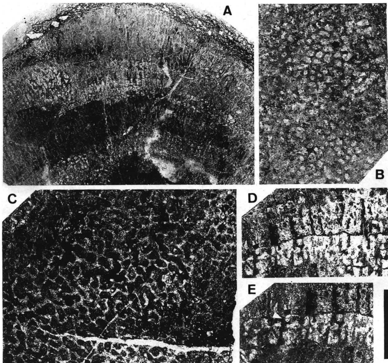
Fig. 4. Sparsisolenia? sp. indet., NMNS PA20408, thin sections. A , longitudinal section of corallum, B , C , transverse sections of corallites, D , E , longitudinal sections of corallites, arrow in E indicates pore protuberance. Scale bar: 7.5 mm in A ; 3 mm in B – D ; 2.5 mm in E .
