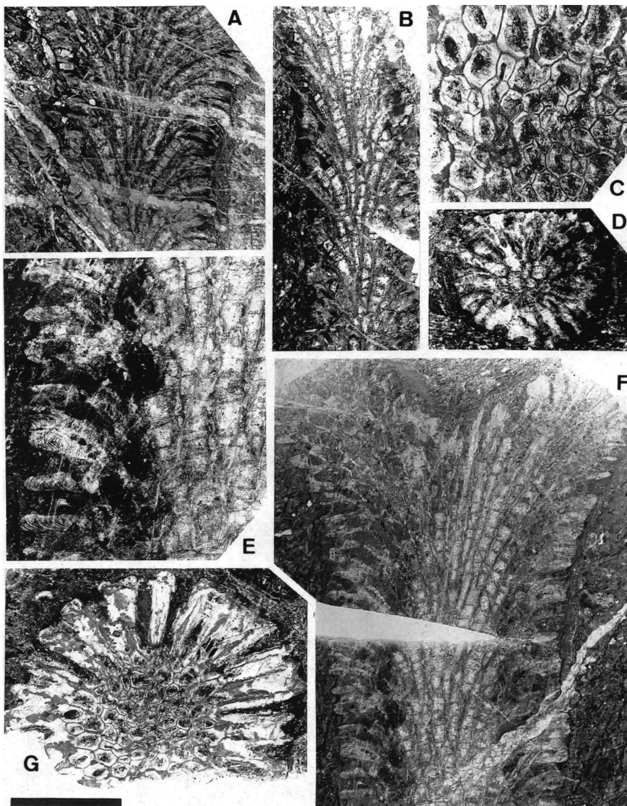
Fig. 8. Thamnoptychia tanimotoi sp. nov., thin sections. A, paratype, NMNS PA20485, longitudinal section of branch. B, paratype, NMNS PA20480, longitudinal section of immature branch. C, E, F, G, holotype, NMNS PA20490; C, partial enlargement of G to show transverse sections of axial corallites, E, partial enlargement of F to show longitudinal sections of corallites, F, longitudinal sections of gerontic branches G, transverse section of gerontic branch. D, paratype, NMNS PA20483, transverse section of branch. Scale bar: 6 mm in A, B, D, F, G; 3 mm in C, E.
