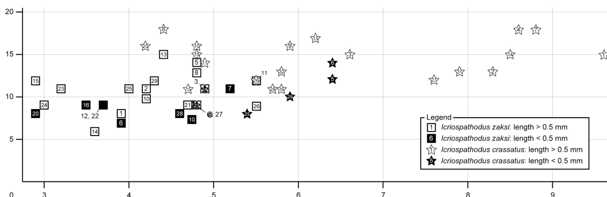
Fig. 6. Scatter diagram showing the relationship between denticle number and length/width ratio in Icriospathodus crassatus and Ic. zaksi . The number inside squares and star marks corresponds to “Number” in Appendix (Iz1–29, Ic1–32). Broken specimens (Iz4, Iz17, Iz19, Ic12, Ic17, Ic18, Ic21, Ic22, Ic30) were unshown.
