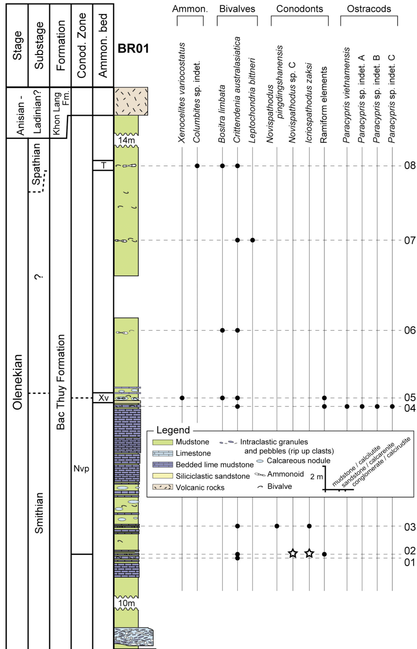
Fig. 4. Columnar section of the Bac Thuy Formation in BR01, Ban Ru area with distributions of ammonoid, bivalve, conodont and ostracoda taxa, modified from Shigeta et al. (2014). Abbreviations: Conod., Conodont; Ammon., Ammonoid; Nvp, Novispathodus pingdingshanensis Zone; Xv, Xenocelites variocostatus beds; T, Tirolites sp. nov. beds.
