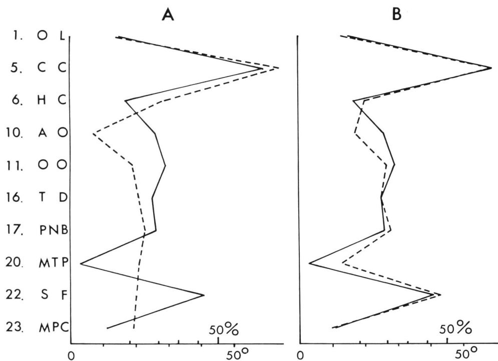
Fig. 2. Graphic comparisons of the incidences of ten traits. Proportions are transformed into angles by FISHER's formula \theta = \arcsin \sqrt{p} .
