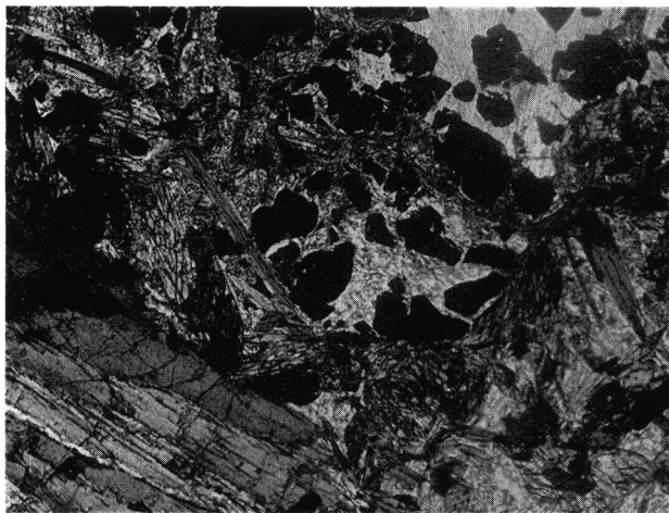
Fig. 3. Photomicrograph of pyrite grains surrounded by chamosite and calcite. One polar. Field view 1.3 \times 1.9 mm.
