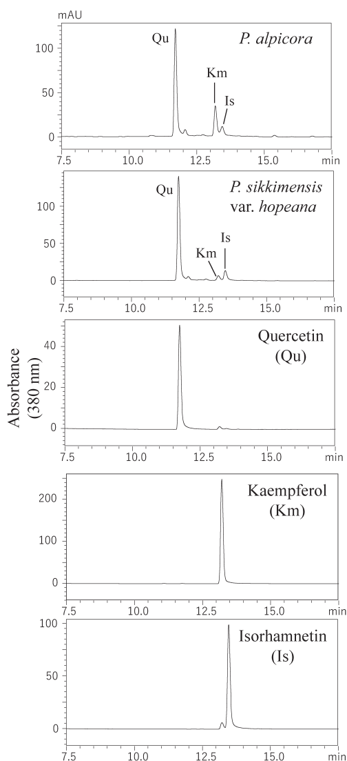
Fig. 8. Aglycone analysis of the flowers of Primura alpicola and P. sikkimensis var. hopeana . These aglycones were compared with authentic flavonols, quercetin (Qu, 11.7 min), kaempferol (Km, 13.2 min) and isorhamnetin (Is, 13.5 min) by HPLC.
