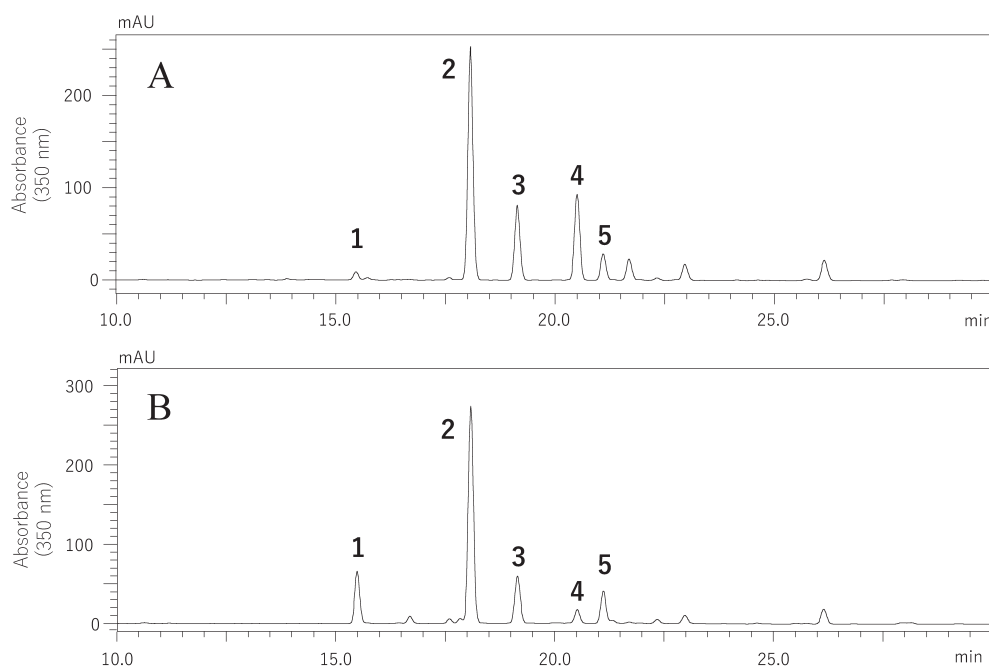
Fig. 7. HPLC analysis of the flowers of Primura alpicola (A) and P. sikkimensis var. hopeana (B). 1 = quercetin 3- O -xylosyl-(1→2)-[rhamnosyl-(1→6)- O -glucoside] (15.5 min), 2 = quercetin 3- O -rutinoside (18.1 min), 3 = quercetin 3- O -glucoside (19.1 min), 4 = kaempferol 3- O -rutinoside (20.5 min), 5 = isorhamnetin 3- O -rutinoside (21.1 min).
