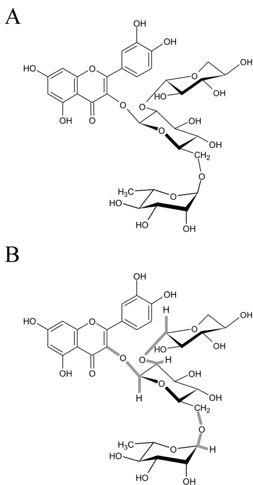
Fig. 2. Quercetin 3- O -xylosyl-(1→2)-[rhamnosyl-(1→6)-glucoside] ( 1 ). A = Chemical structure. B = Significant HMBC correlations were shown as the greyed lines.
