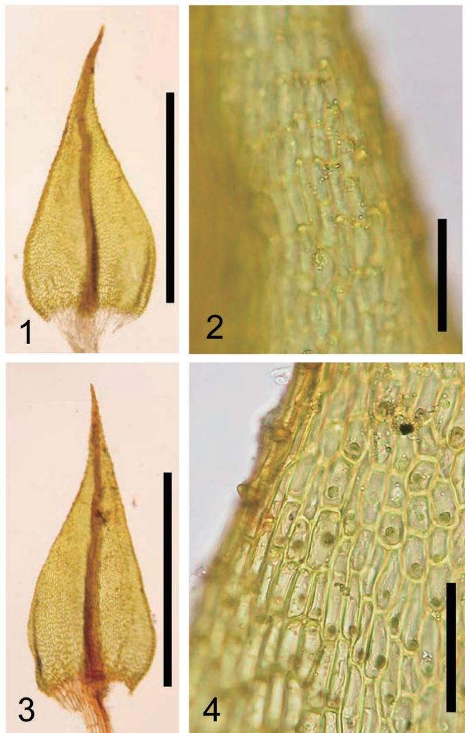
Fig. 2. Philonotis trachyphylla Dixon & Badwh. (Higuchi 19487). 1, 3. Leaves. Scale bar = 1 mm. 2. Ventral surface of cells at upper part of leaf. Scale bar = 50 µm. 4. Dorsal surface of cells at upper part of leaf. Scale bar = 50 µm.
