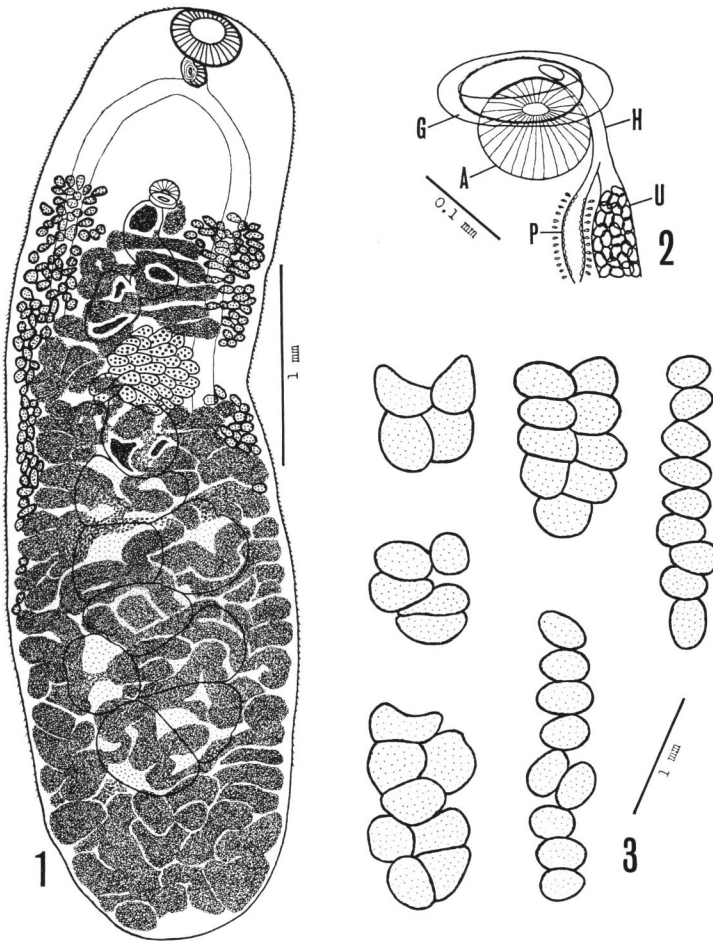
Figs. 1-3. Siphodera gurukun sp. nov. 1. Entire worm, ventral view (NSMT-PI 1280). 2. Terminal genitalia, ventral view (NSMT-PI 2098). A, acetabulum; G, acetabulogenital pouch; H, hermaphroditic duct; P, pars prostatica; U, uterus. 3. Arrangement of testes, ventral view.
