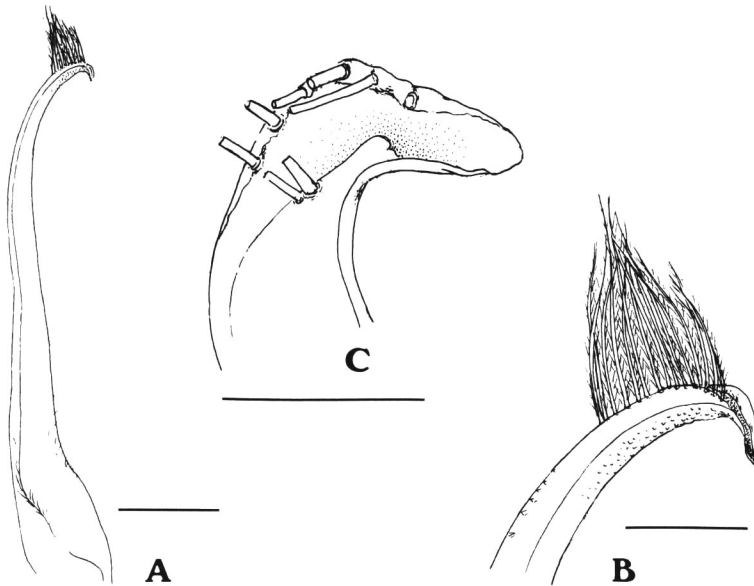
Fig. 3. First male pleopods of holotypes of Atergatis interruptus sp. nov. (A-B) and Meriola corallina sp. nov. (C). Scale for A=5 mm; scales for B and C=1 mm.
