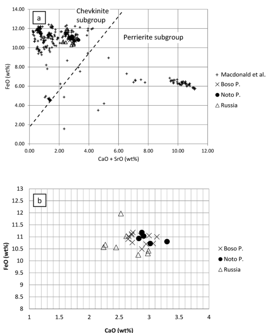
Fig. 4. An empirical FeO vs. (CaO + SrO) compositional variation of chevkinite-(Ce) from the Boso and Noto peninsulas and from Far East Russia. (a) Comparison of the present samples with chevkinite-group minerals from Russia and Mongolia (Macdonald et al. , 2012). (b) Enlarged plot of the present samples. The FeO wt% is total Fe expressed as \text{Fe}^{2+} .
