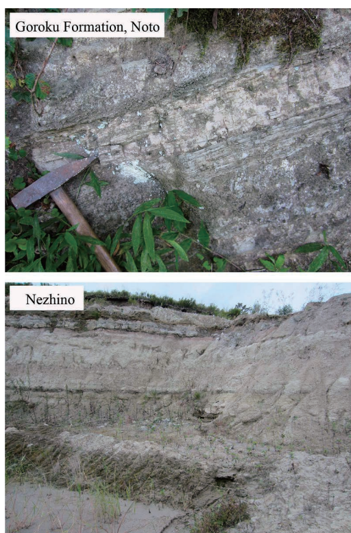
Fig. 2. Outcrop of Chevkinite-bearing tuff in the Goroku Formation from the Noto Peninsula and Monazite-bearing tuff from Nezino in Primorye, Far East Russia.
