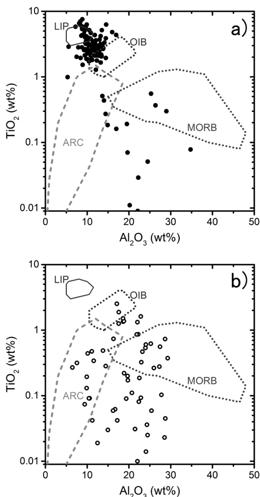
Fig. 4. \text{Al}_2\text{O}_3 vs. \text{TiO}_2 compositional relationships of detrital spinels from (a) main part of the Samarka Belt (RPM01, 04 and 06), and (b) the coastal part of the Samarka Belt and Taukha Belt (RPM40, 47, 48). The discriminations made from the mid-ocean ridge basalt (MORB), ocean-island basalt (OIB), large igneous province (LIP) and island-arc margins (ARC) are after Kamenetsky et al. (2001)
