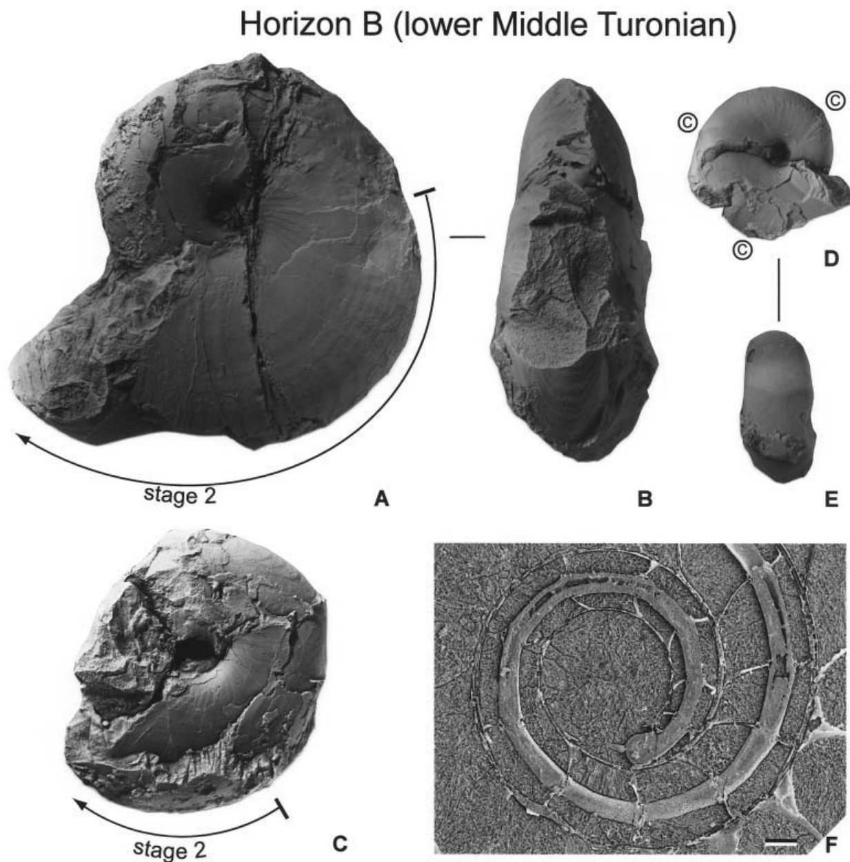
Figure 5. “ T. subcostatus ” collected from horizon B, lower Middle Turonian. A, B. KUM. MM. TN. 039. OT1035. C. KUM. MM. TN. 042. OT1034. D, E. KUM. MM. TN. 053. OT1035. F. KUM. MM. TN. 064. OT3051. A–C in natural size. D, E, \times 3 . F, scale bar = 0.1 mm. Abbreviations are the same as in Figure 4.
