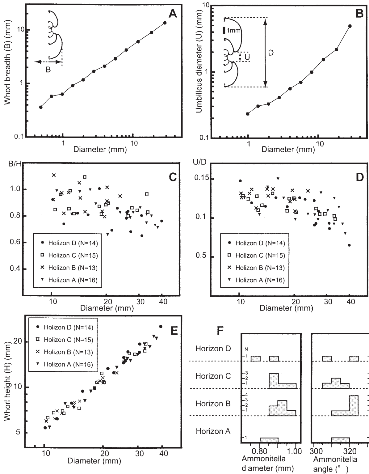
Figure 9. Measurements of " Tragodesmocerooides subcostatus " collected from four horizons. A. Whorl diameter/breadth change with ontogeny in specimen KUM. MM. TN. 009. B. Whorl diameter/umbilicus diameter change with ontogeny in specimen KUM. MM. TN. 009. C. Whorl breadth/Height ratio (B/H) in relation to shell diameter for juvenile to near-adult stage. D. Umbilicus/Diameter ratio (U/D) in relation to shell diameter for juvenile to near-adult stage. E. Whorl diameter/Whorl height relationship. F. Ammonitella diameter and angles from horizon A–D. All parameters do not show chorologically significant changes.
