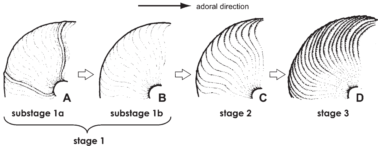
Figure 10. Schematic diagrams illustrating typical shell surface ornament stages and substages in “ Tragodesmocerooides subcostatus ”. A. substage 1a; Desmoceratid-type constriction. B. substage 1b; Almost smooth with fine growth line. C. Stage 2; Weak ribbing. D. Stage 3; Coarse ribbing (diagnostic feature). Not to scale. A black arrow indicates adoral direction.
