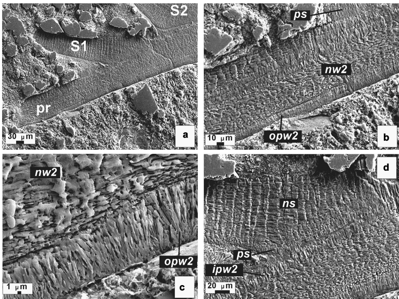
Fig. 14. SEM images of well-preserved Cymatoceras sp. shell structure, including structure of proseptum, M-1 from Madagascar. a – proseptum, b – median section of the shell wall and septum in the 1st whorl, c and d – the details of Fig. 12b and a, respectively. Designations: pr – proseptum, S1 and S2 – 1st and 2nd septa, ps – prismatic layer of the septum, ns – nacreous layer of the septum, nw2 – nacreous layer in the 2nd whorl, opw2 – outer prismatic layer in the 2nd whorl, ipw2 – inner prismatic layer in the 2nd whorl.
