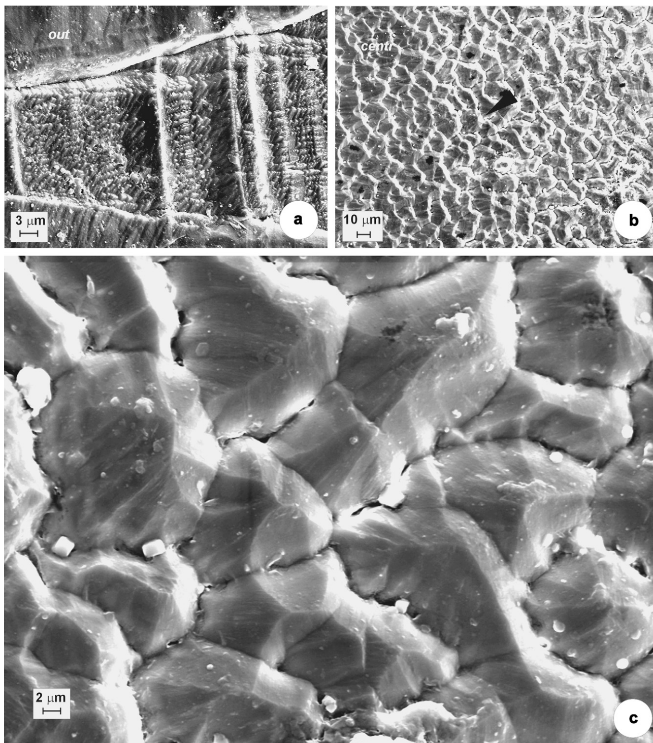
Fig. 9. SEM photomicrographs of belemnite Parahibolites blanfordi (Spengler), longitudinal section of the rostrum In-10e from southern India: a – etched surface shows well-preserved prismatic calcite in another tooth-like locus of the outlying part of the rostrum; b – detail of Fig. 7d shows well-preserved pellets of the central part of the rostrum (granular structure); c – detail of Fig. 9b shows configuration of pellets (grains).
