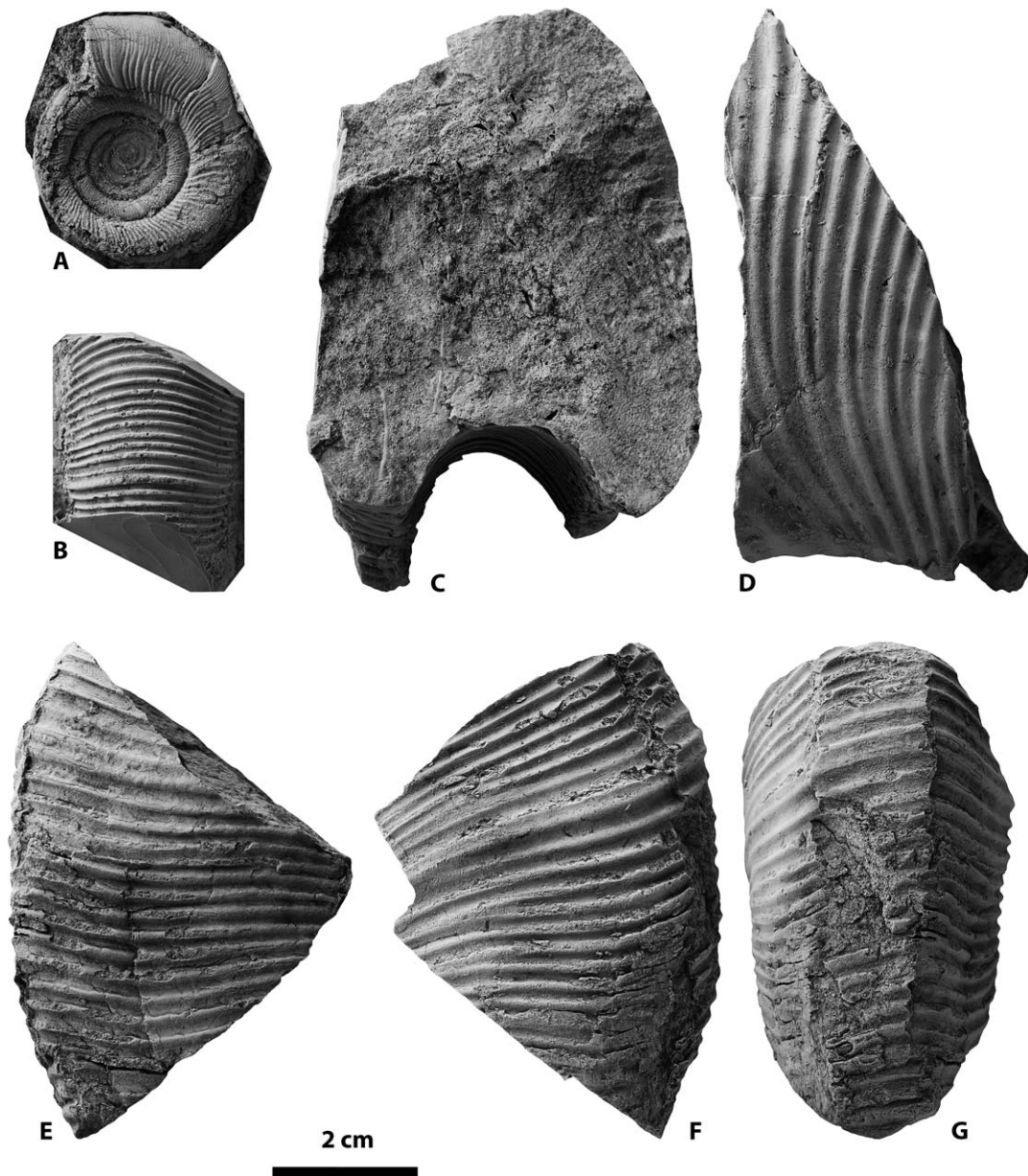
Figure 7. Gaudryceras hobetsense Shigeta and Nishimura sp. nov. from the Nakatombetsu area, Hokkaido. A , NMNS PM23450 (silicon rubber cast), right lateral view; B-D , NMNS PM23451; B , silicon rubber cast of ventral part of previous whorl; C , apertural view; D , right lateral view; E-G , NMNS PM23452; E , left lateral view; F , right lateral view; G , ventral view.
