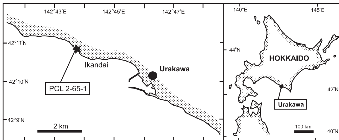
Figure 1. Index map showing collection locality (NMNS PCL 2-65-1) of Morewites sakakibarae Shigeta gen. et sp. nov. in the Urakawa area, Hokkaido.
