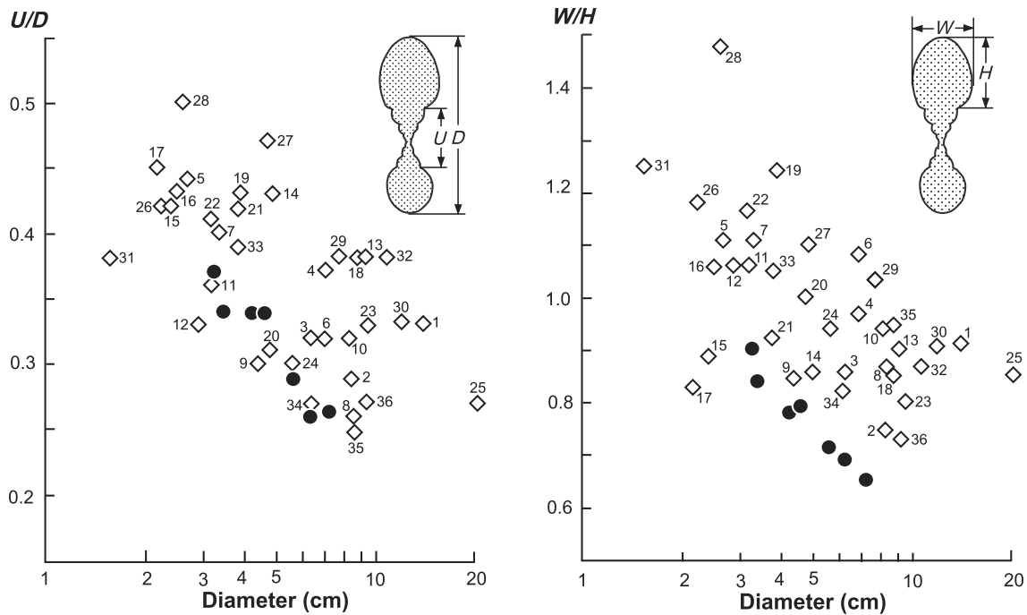
Figure 7. Scatter diagrams of umbilical diameter/shell diameter ( U/D ) versus shell diameter ( D ) and whorl width/whorl height ( W/H ) versus shell diameter ( D ) for seven specimens of Anagaudryceras compressum Shigeta and Nishimura sp. nov. (black circles) and thirty-six selected type (holotype and lectotype) specimens assigned to Anagaudryceras by Klein et al. (2009) (white squares). Klein et al. (2009) listed fifty-three species of Anagaudryceras , but shell measurements for fifteen of the species are not provided and the generic assignment for two species is incorrect: A. matsumotoi (Grabovskaya in Zakharov et al. , 1981) clearly belongs to Zelandites and A. rouvillei (Grossouvre, 1894) belongs to Pseudophyllites Kossmat, 1895. Number in each square corresponds as follows. 1, A. aureum (Anderson, 1958), holotype; 2, A. aurarium (Anderson, 1938), holotype; 3, A. cappsi (Imlay, 1960), holotype; 4, A. coagmentatum (Collignon, 1963), holotype; 5, A. crenatum (Marshall, 1926), holotype; 6, A. enigma (Matsumoto et al. , 1972), holotype; 7, A. filicinatum (Whiteaves, 1876), lectotype; 8, A. howarthi Matsumoto, 1995, holotype; 9, A. involvulum (Stoliczka, 1865), holotype; 10, A. limatum (Yabe, 1903), holotype; 11, A. madraspatanum (Stoliczka, 1865), lectotype; 12, A. matsumotoi Morozumi, 1985; 13, A. mikobokense Collignon, 1956, holotype; 14, A. multiplexum (Stoliczka, 1865), holotype; 15, A. nanum Matsumoto, 1985, holotype; 16, A. particostatum (Marshall, 1926), lectotype; 17, A. ? pauli (Coquand, 1862), holotype; 18, A. politissimum (Kossmat, 1895), holotype; 19, A. pulchrum (Crick, 1907), holotype; 20, A. pulvinatum (Collignon, 1964), holotype; 21, A. revelatum (Stoliczka, 1865), holotype; 22, A. sacya (Forbes, 1846), holotype; 23, A. sakalavum (Collignon, 1949), holotype; 24, A. salinarium (Douville, 1931), holotype; 25, A. seymouriense Macellari, 1986, holotype; 26, A. subsacya (Marshall, 1926), lectotype; 27, A. tennenti Henderson, 1970, holotype; 28, A. tenuilineatum (Hoepen, 1921), holotype; 29, A. tetragonum Matsumoto and Kanie, 1985, holotype; 30, A. utaturensis Shimizu, 1935, holotype; 31, A. valudayurensis (Kossmat, 1895), holotype; 32, A. whitneyi (Gabb, 1869), holotype; 33, A. woodsi Henderson, 1973, holotype; 34, A. yamashitai (Yabe, 1903), holotype; 35, A. yokoyamai (Yabe, 1903), holotype; 36, A. yokoyamaiforme Collignon, 1969, holotype.
