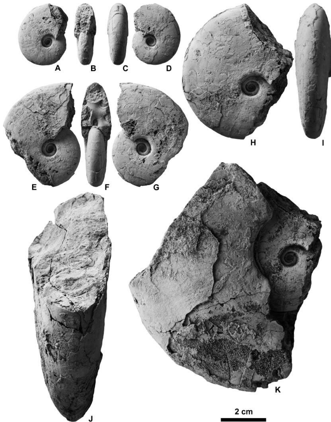
Figure 9. Churkites egregius Zharnikova and Okuneva in Okuneva (1990), NMNS PM35000, from the Smolyaninovo section. A–I , inner whorls of J and K; A, H, E , left lateral views; B, F , apertural views; C, I , ventral views; D, G , right lateral views; J , ventral view; K , left lateral view.
