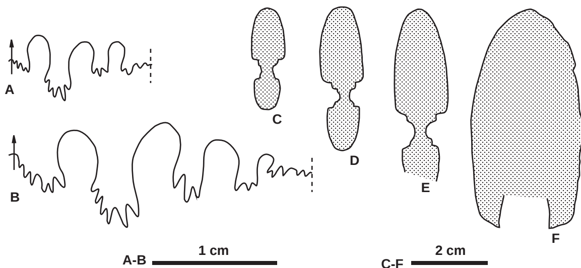
Figure 8. Suture lines (A, at H = 10 mm; B, at H = 27 mm) and whorl cross sections (C–F) of Churkites egregius Zharnikova and Okuneva in Okuneva (1990), NMNS PM35000, from the Smolyaninovo section. Solid and broken lines indicate position of the siphuncle and umbilical seam.
