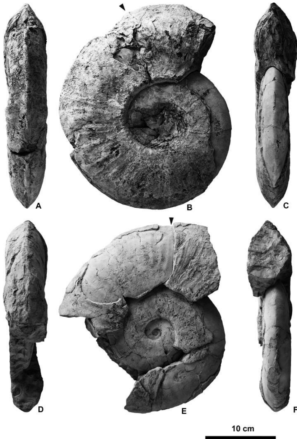
Figure 11. Churkites egregius Zharnikova and Okuneva in Okuneva (1990) from the Smolyaninovo section. A–C , NMNS PM35004; A , ventral view; B , left lateral view; C , apertural view; D–F , NMNS PM35003; D , ventral view; E , left lateral view; F , apertural view. Arrow indicates position of last septum.
