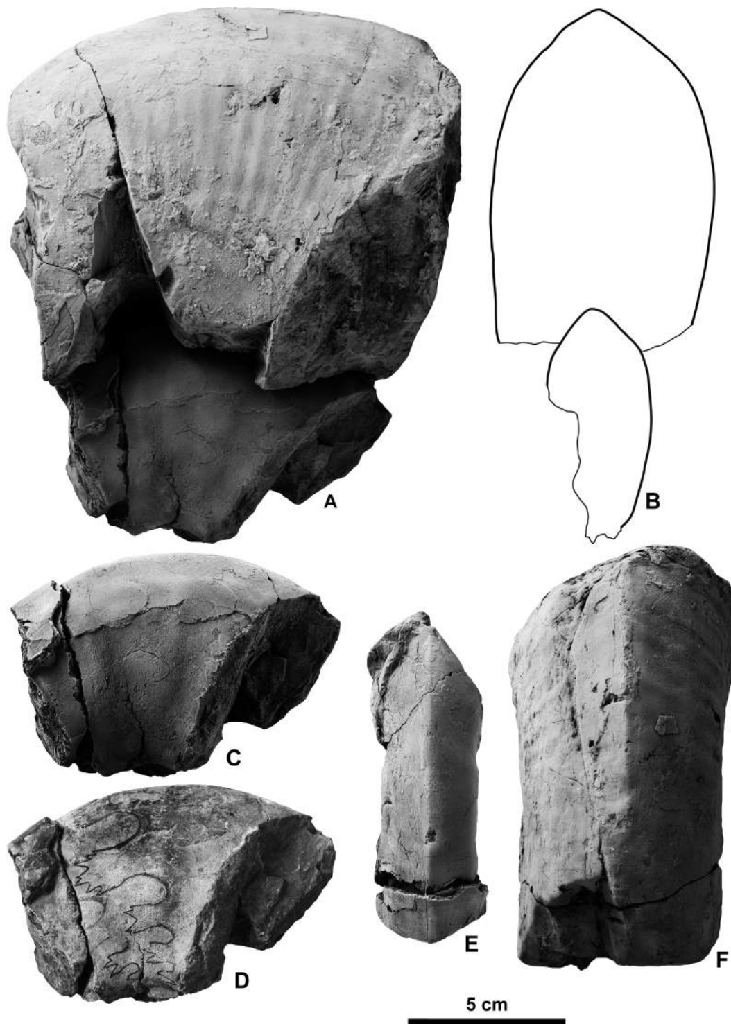
Figure 7. Holotype of Churkites egregius Zharnikova and Okuneva in Okuneva (1990), from the Lower Triassic (upper Smithian?) in the Artiomyvka River section. A, C, E, F , plaster cast of the holotype, NMNS PM35014; A , left lateral view; C , left lateral view of the inner whorl of A ; E , ventral view of C ; F , ventral view of A ; B , whorl cross section; D , left lateral view of the inner whorl of the holotype, CGM 1/10379.
