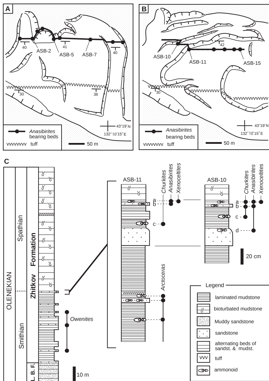
Figure 3. Localities (A, B) of the Artyom section and horizons (C) from which specimens of Churkites were collected. Sketch maps A and B of the quarry were made in 2005–2008 and 2011–2012 respectively. The 50–60 cm thick Anasibirites -bearing beds and the 30 cm thick white vitric tuff bed are widely traceable in the quarry. Specimens of Churkites were collected from ABS-2, 5, 7, 10a, b, c, 11c and 15. L.B.F., Lazurnaya Bay Formation.
