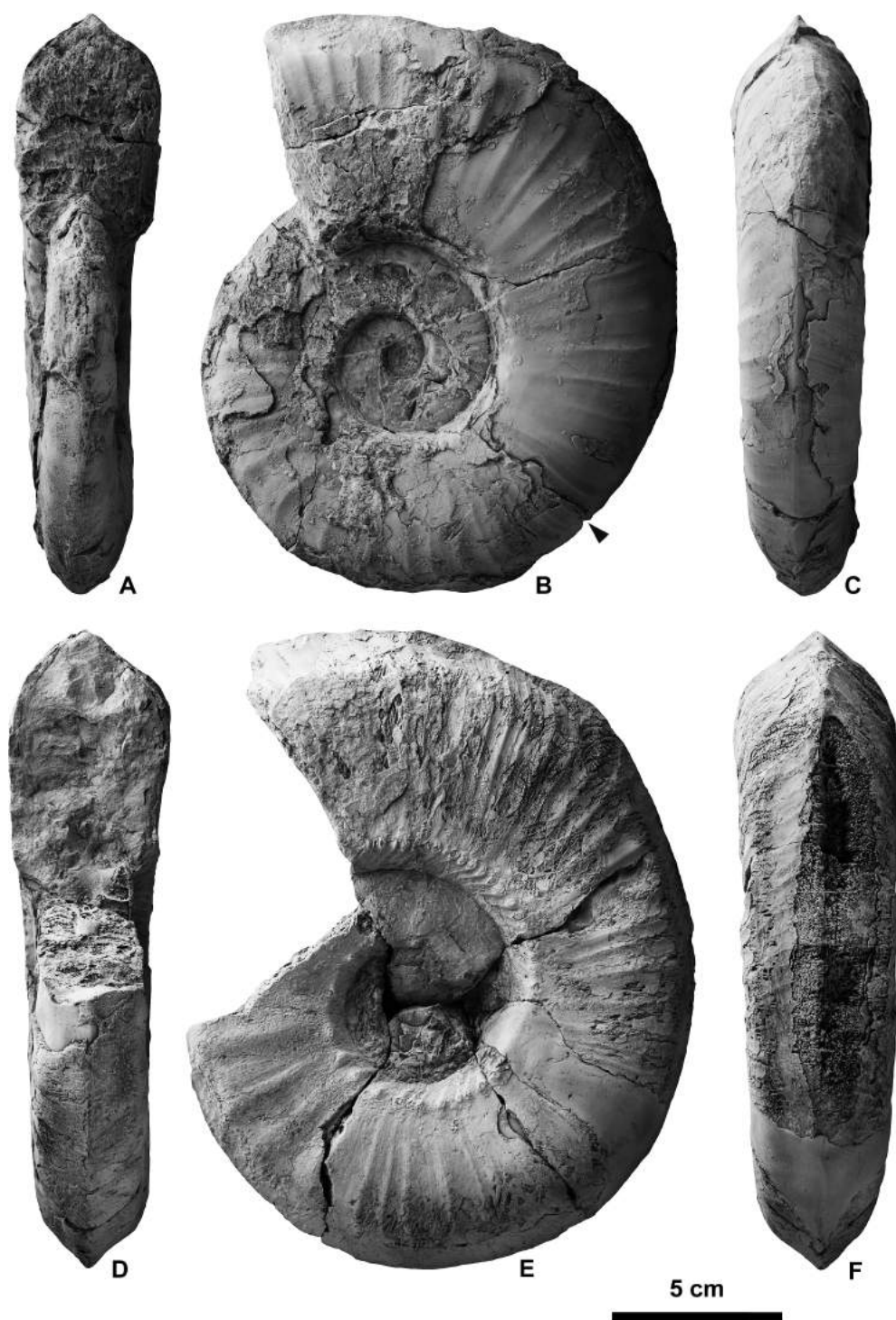
Figure 10. Churkites egregius Zharnikova and Okuneva in Okuneva (1990) from the Smolyaninovo section. A–C , NMNS PM35001; A , apertural view; B , right lateral view; C , ventral view; D–F , NMNS PM35002; D , apertural view; E , right lateral view; F , ventral view. Arrow indicates position of last septum.
