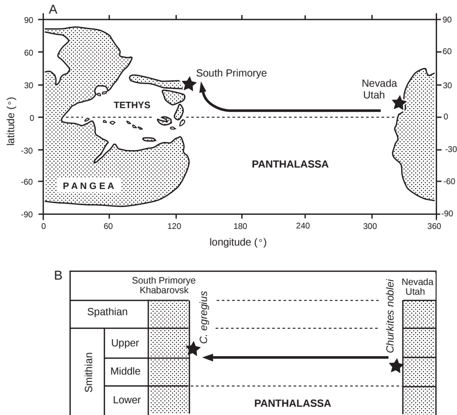
Figure 13. Paleogeographical (A) and stratigraphical position (B) of Churkites . Churkites most likely originated from Arctoceras tuberculatum on the eastern side of the Panthalassa during the middle Smithian, crossed the Panthalassa and gave rise to C. egregius on the western side of the Panthalassa during the late Smithian. Paleomap modified after Péron et al. (2005), Brayard et al. (2006) and Shigeta et al. (2009).
