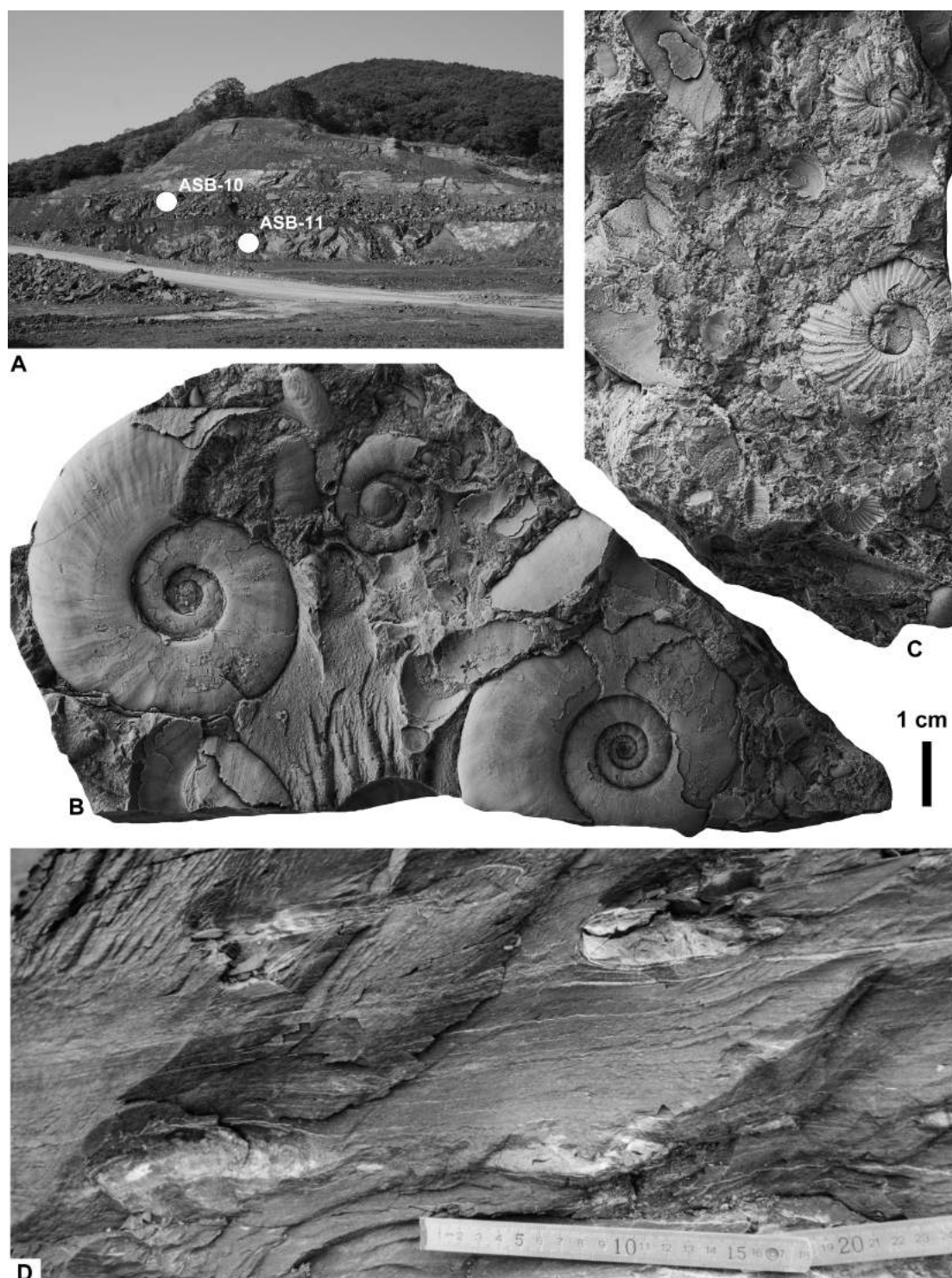
Figure 4. Ammonoid mode of occurrence in the Artyom section. A , Distant view of northern side of quarry; B , Xenoceltites -bearing mudstone of the Zhitkov Formation at ASB-10a; C , Anasibirites -bearing fine-grained sandstone of the Zhitkov Formation at ASB-10b; D , Large-sized Arctoceras of middle Smithian age in finely laminated mudstone; mode of occurrence is very similar to that of Churkites at ASB-10c. Although Churkites only occurs rarely with Anasibirites at ASB-10B, it is relatively abundant at ASB-10a and ASB-10c.
