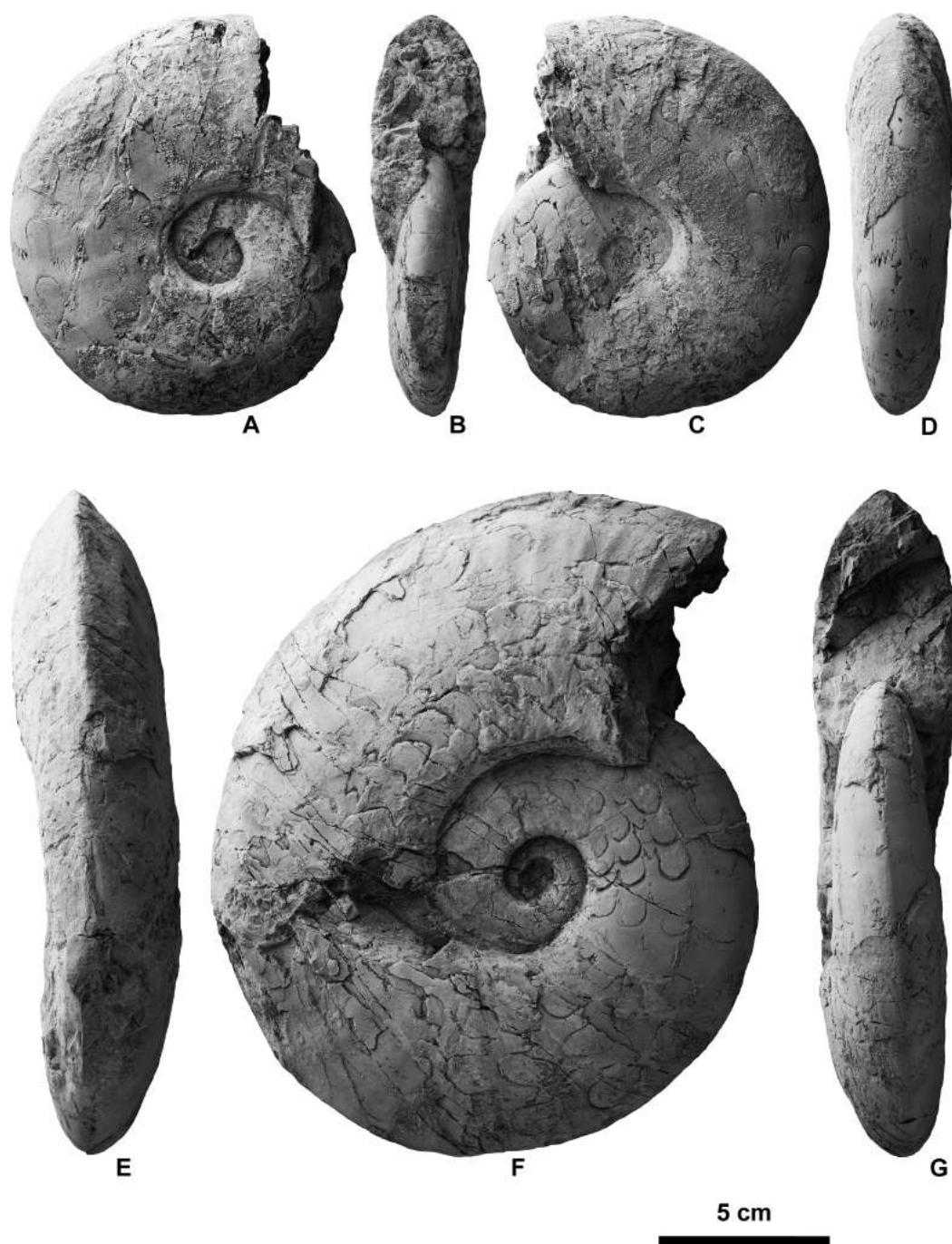
Figure 12. Churkites egregius Zharnikova and Okuneva in Okuneva (1990) from the upper Smithian Anasibirites beds at ASB-11c in the Artyom section. A–D , NMNS PM35011; A , left lateral view; B , apertural view; C , right lateral view; D , ventral view; E–G , NMNS PM35012; E , ventral view; F , left lateral view; G , apertural view.
