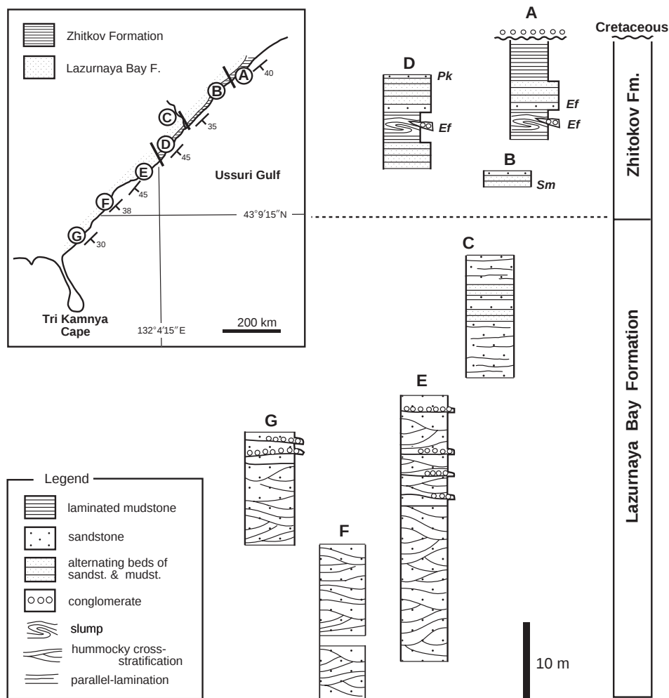
Figure 5. Columnar sections of the Lower Triassic in the Tri Kamnya section. Ef, Euflemingites prynadai ; Pk, Palaeokazakhstanites ussuriensis ; Sm, Shamaraites schamarensis .
