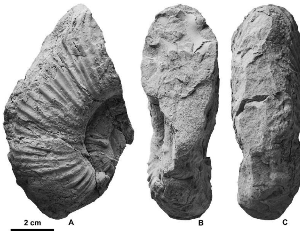
Figure 15. Canadoceras multicosstatum Matsumoto, 1954, NMNS PM35027, from Loc. 3 in the Chinomigawa Formation. A , left lateral view; B , apertural view; C , ventral view.
