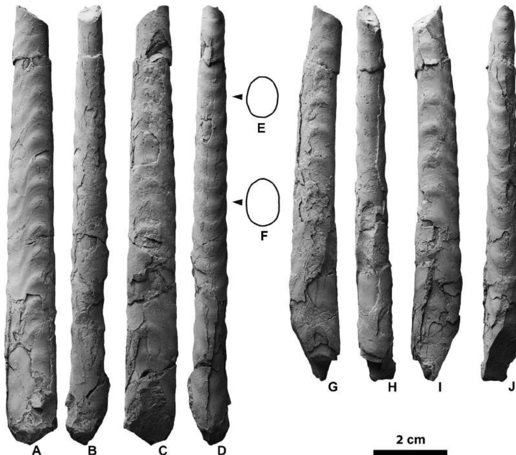
Figure 27. Baculites subanceps Haughton, 1925 from Loc. 14 in the Chinomigawa Formation. A–F , HMG-1675; A , lateral view; B , dorsal view; C , lateral view rotated 90 degrees from A ; D , ventral view; E , whorl cross section at H = 11.2 mm; F , whorl cross section at H = 12.8 mm; G–J , HMG-1676; G , lateral view; H , dorsal view; I , lateral view rotated 90 degrees from G ; J , ventral view.
