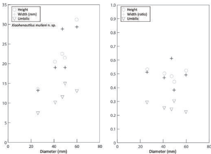
FIGURE 13. Scatter diagrams of H, W and U, and H/D, W/D and U/D for Xiaohenautilus mullenii n. sp.
