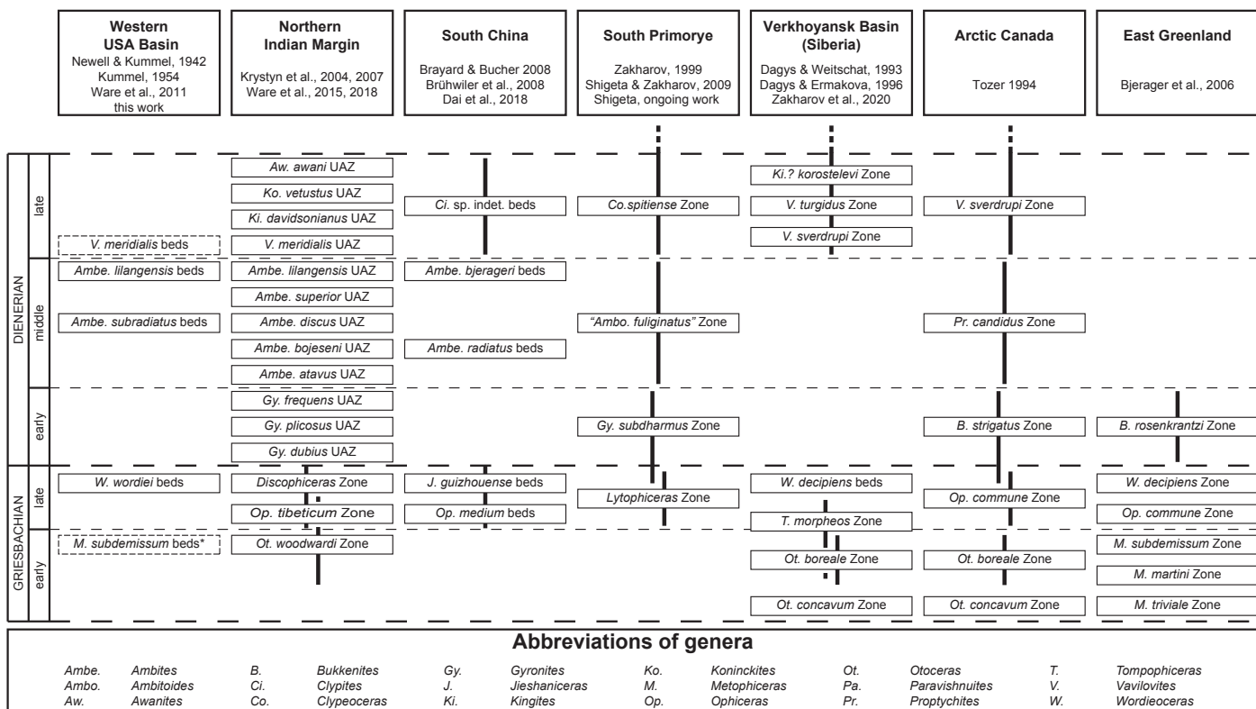
FIGURE 6. Induan ammonoid zonation of the western USA basin and correlation with other global occurrences. Bold vertical black bars represent uncertain correlation. Dashed line boxes encompassing Vavilovites meridialis beds and Metophiceras subdemissum beds of western USA basin represent uncertain stratigraphic occurrences within late Dienerian and early Griesbachian, respectively. Similarly, asterisk marking M. subdemissum beds denotes uncertain ammonoid identification. Note: Ongoing work by Ware is expected to significantly modify the zonation of Bjerager et al., (2006) for East Greenland. UAZ = Unitary Association Zone.
