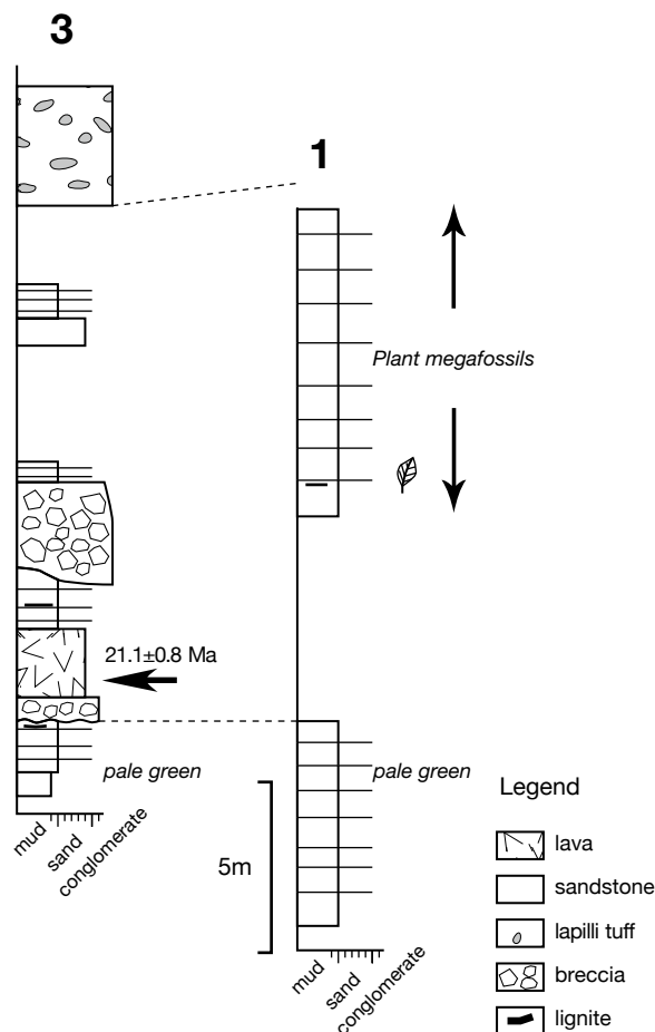
FIGURE 2. Stratigraphic columnar section at Locs. 1 and 3, showing stratigraphic levels of a sample for ^{40}\text{Ar} - ^{39}\text{Ar} analysis and possible plant megafossil horizons. Two columnar sections are correlated with each other, based on the greenish mudstone at the base of each locality and the absence of lapilli tuff at the top of the Loc. 1. A leaf mark points the plant megafossil horizon collected by the author.
