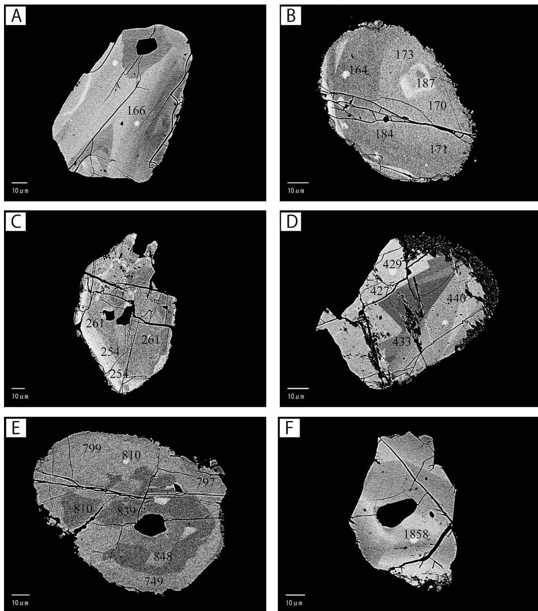
Fig. 4. Back-scattered images of detrital monazites with various ages. A & B: monazites with ages less than 200 Ma. C: monazite with age around 260 Ma. D & E: rare monazites with 430 Ma and 800 Ma, respectively. F: monazite with 1860 Ma. The number in each grain shows monazite age (Ma).
