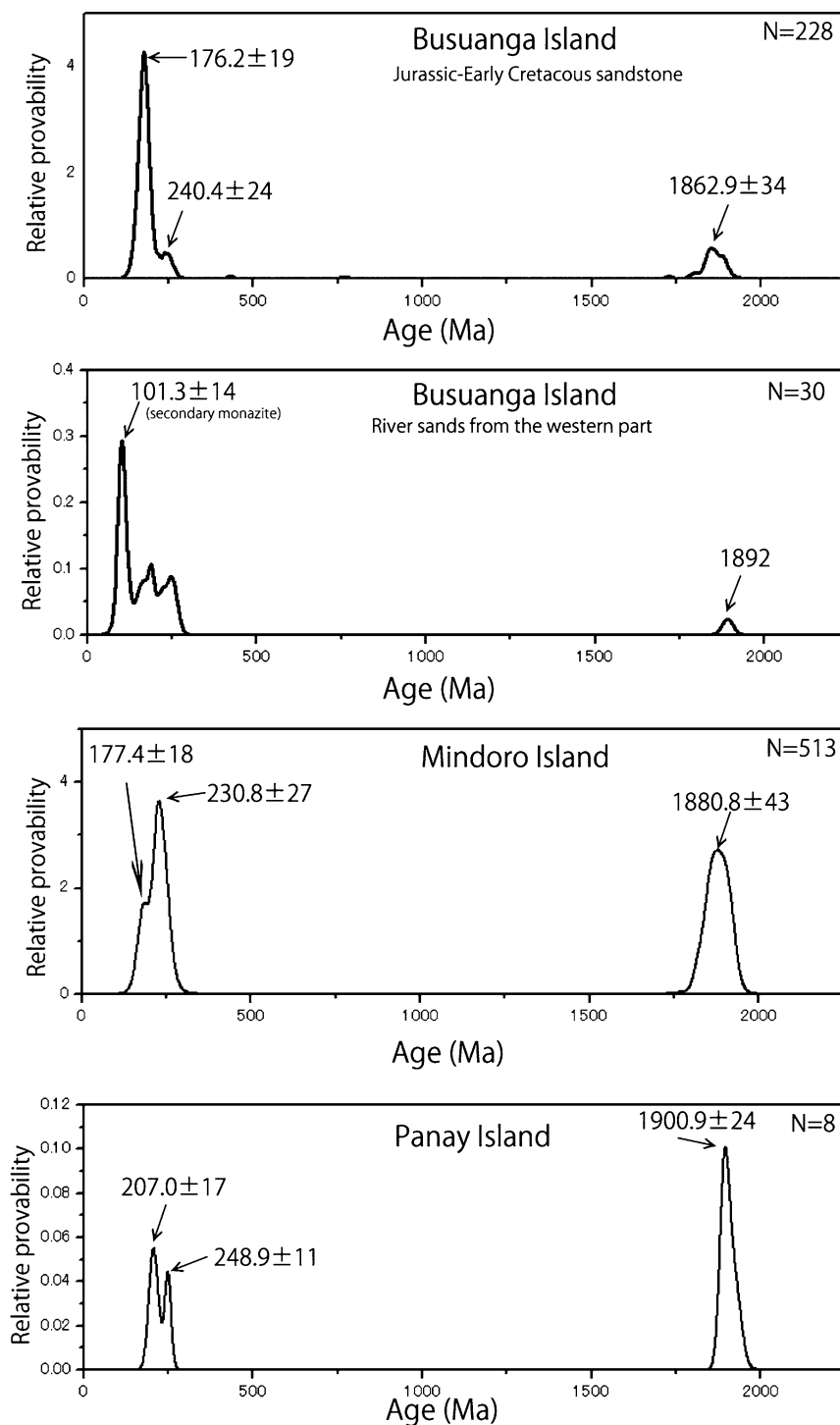
Fig. 6. Probability distribution diagrams of monazite ages in the sandstones and sands from Busuanga, Mindoro, and Panay islands. Numerical value (n) denotes the number of analyzed monazite grains.
