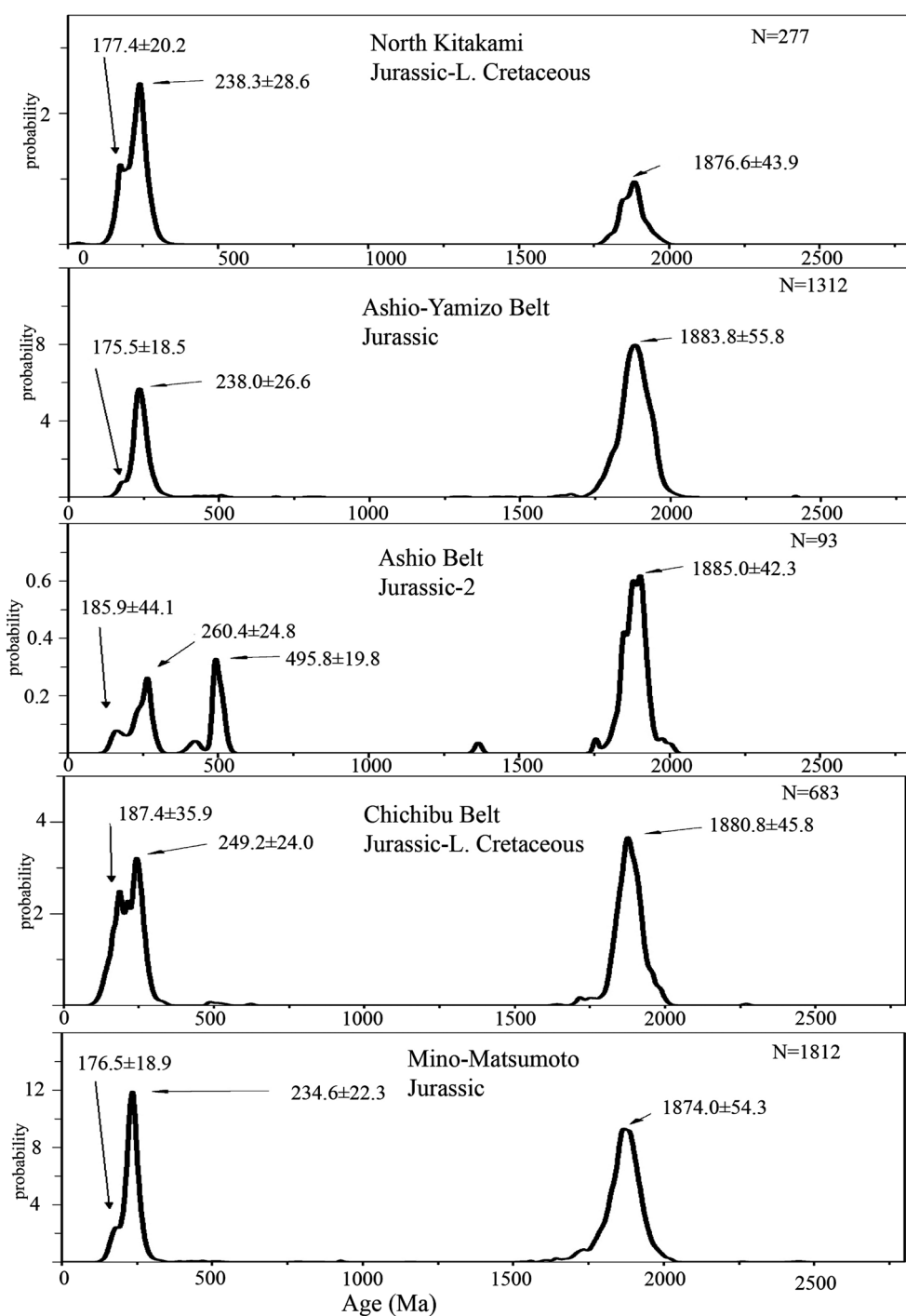
Fig. 5. Probability distribution of ages of detrital monazites in the sandstones from the accretionary complexes in the north and central part of the Japanese Islands. The numerical value (n) denotes the number of analyzed monazite grains.
