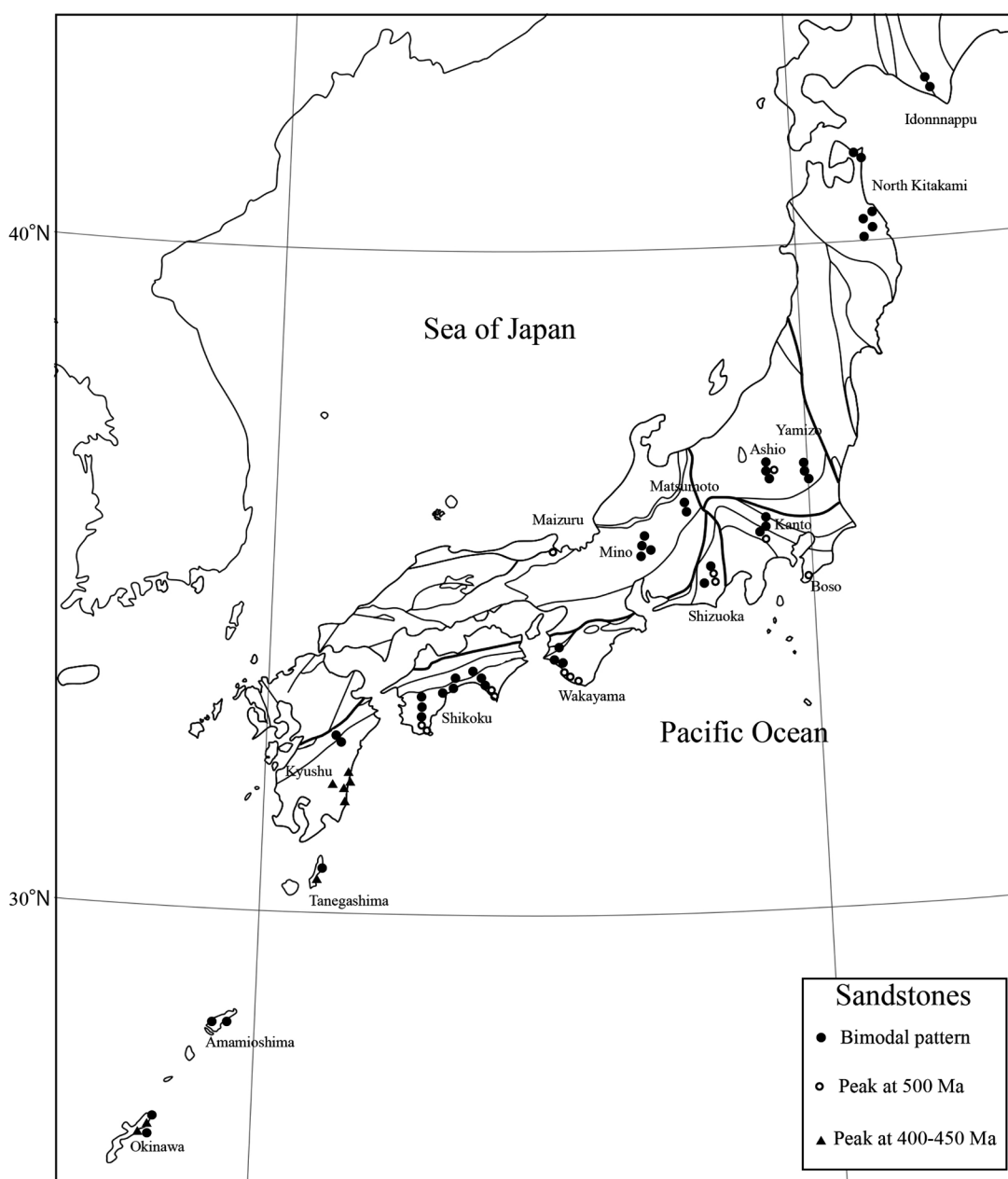
Fig. 3. Sampling sites of sandstones in the accretionary complexes including previously studied sites.
