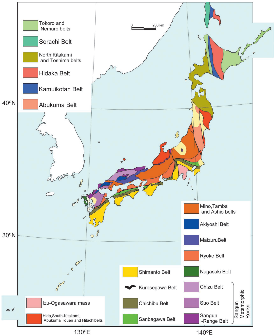
Fig. 1. Geological division of the basement rocks in the Japanese Islands.
