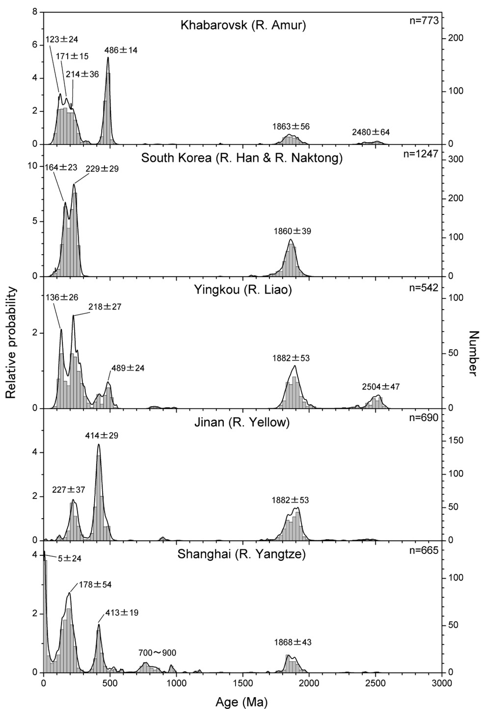
Fig. 7. Probability distribution of monazite ages in the sands from the major rivers in East Asia (After Yokoyama et al. , 2007). The numerical value (n) denotes the number of analyzed monazite grains.
