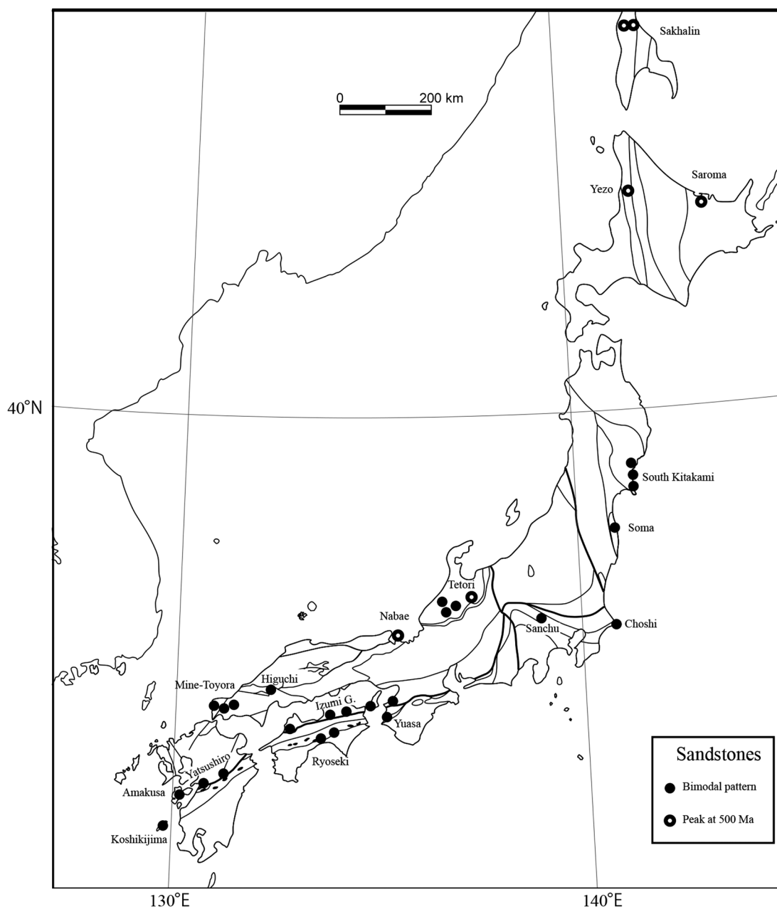
Fig. 4. Sampling sites of sandstones in the non- and shallow-marine sequences including previously studied sites.
