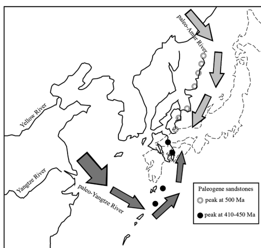
Fig. 10. Model of sediment supplies from the continent to the Paleogene accretionary complex of the Shimanto Belt.
