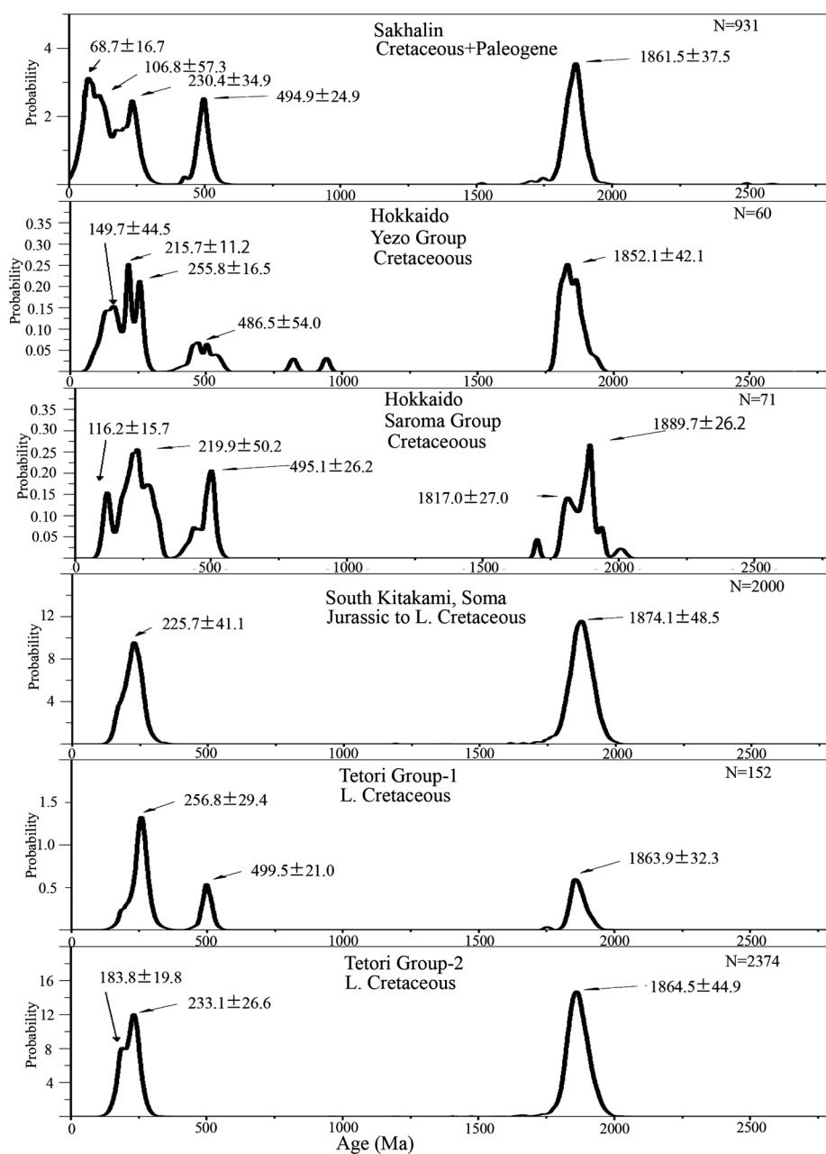
Fig. 8. Probability distribution of ages of detrital monazites in the sandstones from the non- and shallow-marine sequences in Sakhalin, Hokkaido, south Kitakami and Tetori. The numerical value (n) denotes the number of analyzed monazite grains.
