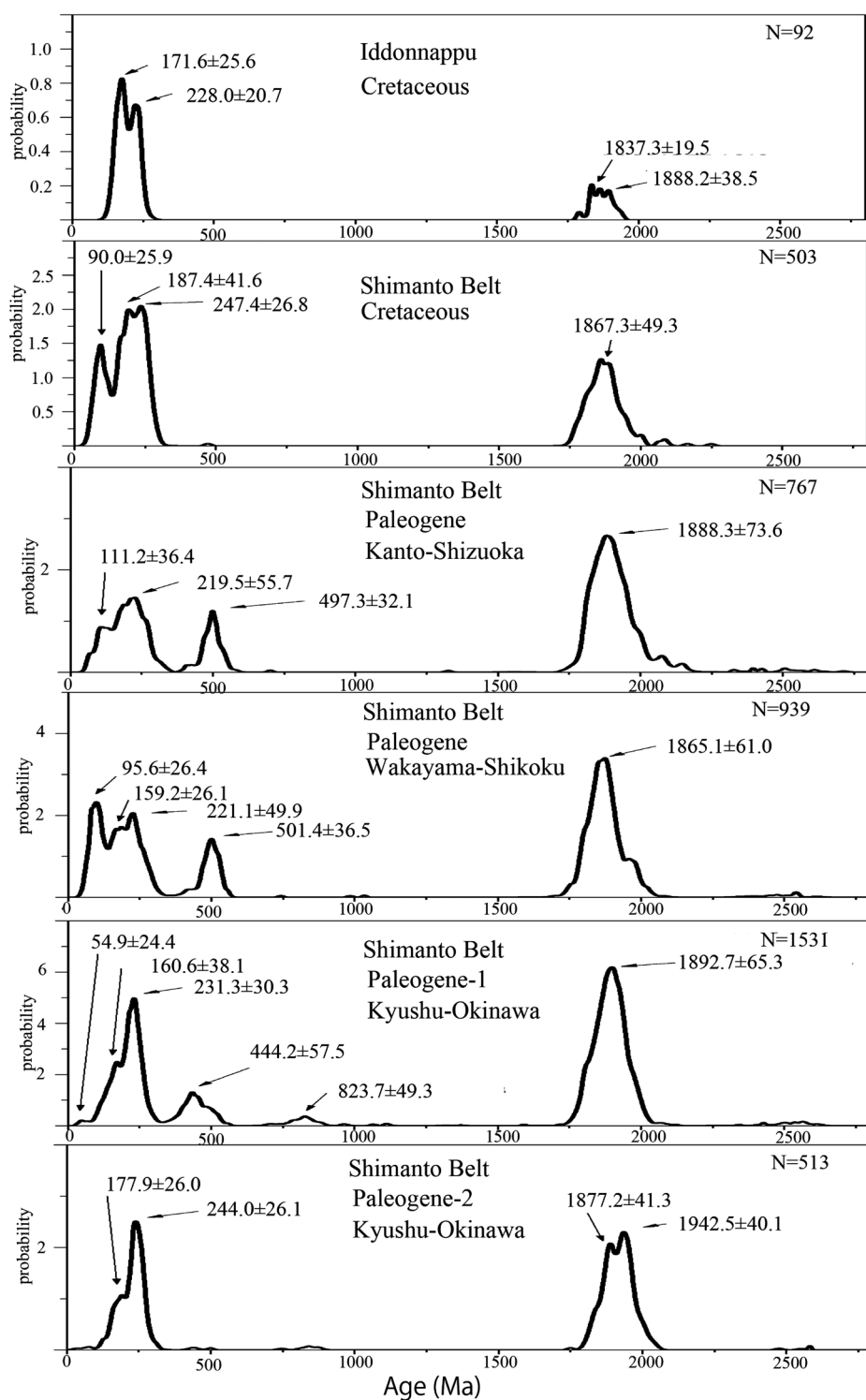
Fig. 6. Probability distribution for the ages of detrital monazites in the sandstones from the Iddonnappu Belt and Shimanto Belt. The numerical value (n) denotes the number of analyzed monazite grains.
