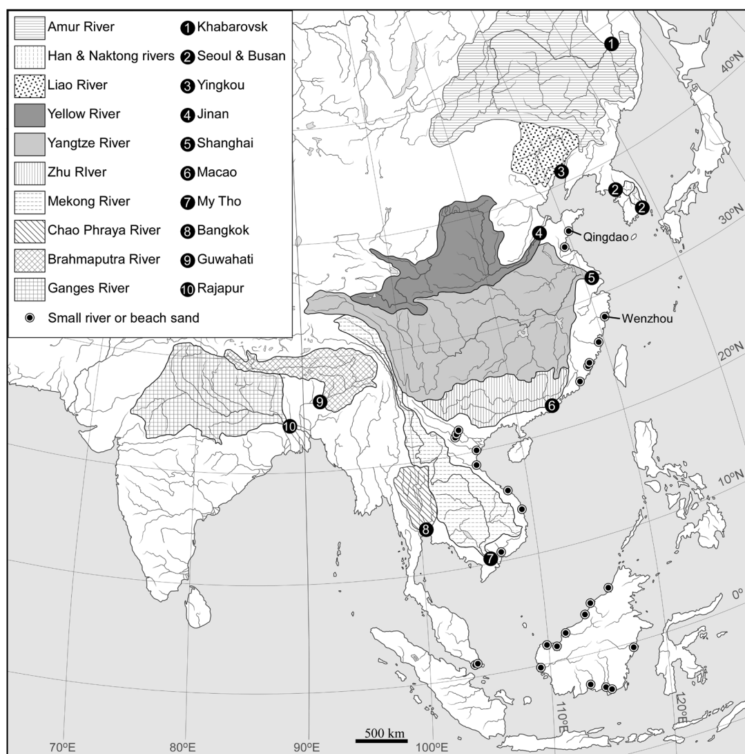
Fig. 2. Sampling localities of sands from the rivers in Asia. The age data of the sands were already published by Yokoyama et al. , 2007, 2008, 2010a, 2010b, 2012 & 2015).
