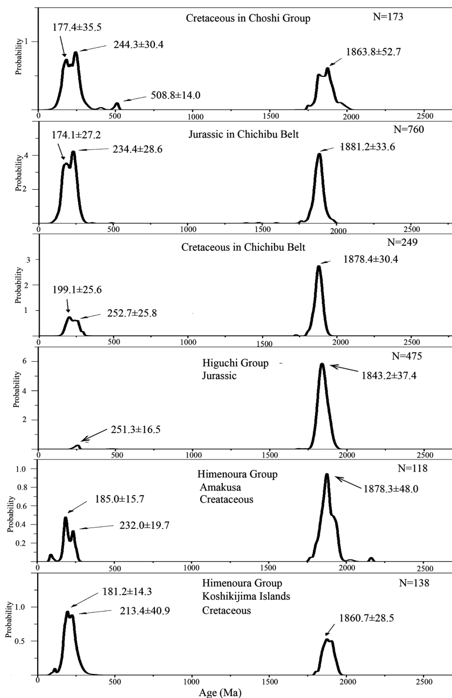
Fig. 9. Probability distribution of the ages of the detrital monazites in the Jurassic and Cretaceous sandstones from the non- and shallow-marine sequences in Chichibu Belt, Higuchi Group and Himenoura Group. The numerical value (n) denotes the number of analyzed monazite grains.
