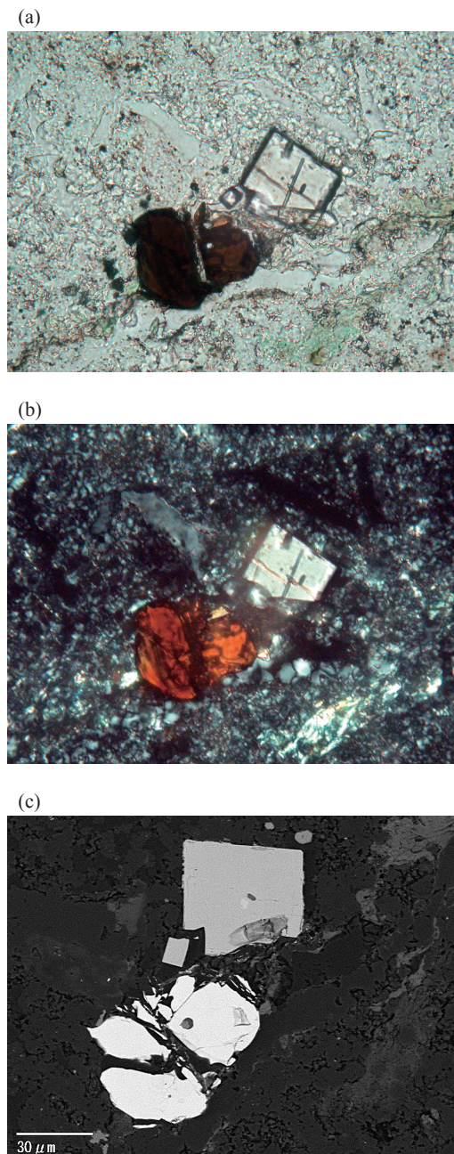
Fig. 2. Photomicrographs [plane polarized light (PPL) (a) and crossed polars (CPL) (b)] and back scattered electron image (c) of chevkinite-(Ce) [brown in PL and pale gray in BSE] and zircon [colorless in PL and gray in BSE] in the rhyolitic tuff.
