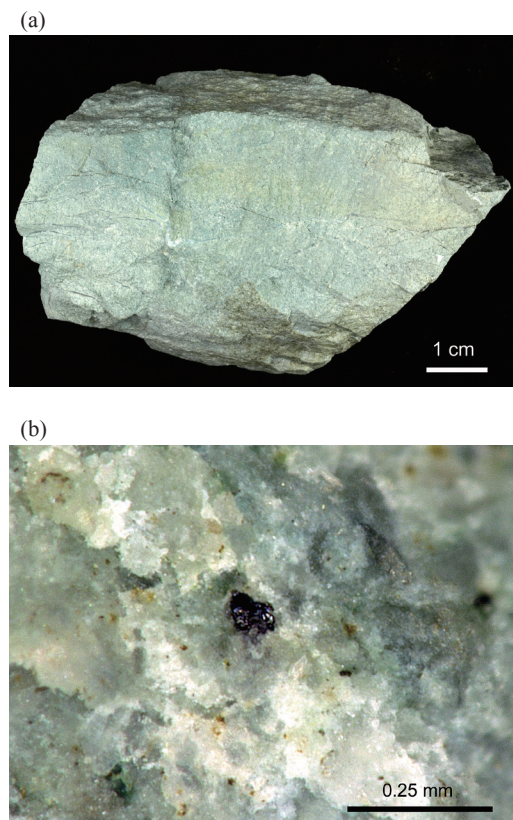
Fig. 1. The appearance of pale green rhyolitic tuff (a) and the close up view of black crystal of chevkinite-(Ce) of the rhyolitic tuff (b).
