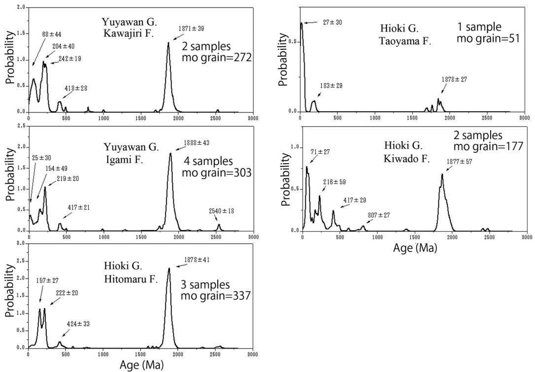
Fig. 5. Relative probability distribution diagrams of monazite ages of the sandstones from the Nagato area.
