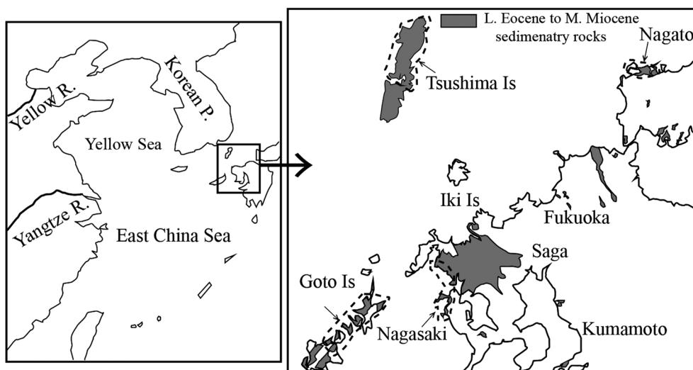
Fig. 1. Map showing sampling regions in the northern Kyushu and western Chugoku provinces; Tsushima Islands, Goto Islands, Nagato area and Nagasaki area.
