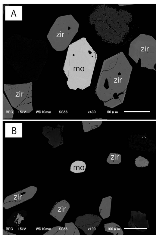
Fig. 3. Back-scattered electron images of detrital monazite grains in the tuffaceous sample (SB-10) from the Nishiusuki Group. A: a euhedral monazite with volcanic glass inclusions, mo = monazite, zir = zircon. B: a rounded detrital monazite.
