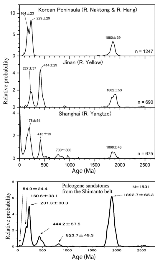
Fig. 7. Relative probability distribution diagrams of monazite ages of the sands from the Korean Peninsula, Yellow and Yangtze rivers (after Yokoyama et al. , 2007). The probability diagram for the Paleogene sandstones from the Shimanto Belt is from Yokoyama (2016).
