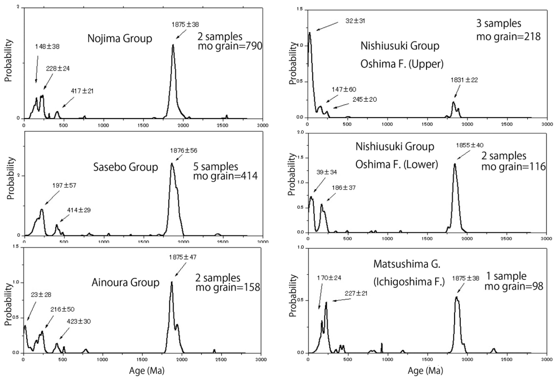
Fig. 6. Relative probability distribution diagrams of monazite ages of the sandstones from the Nagasaki area.
