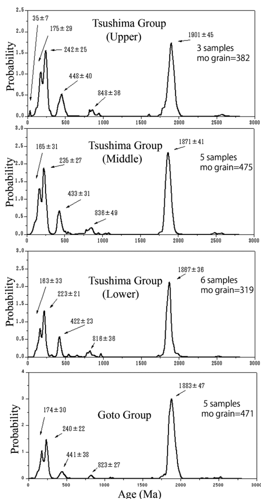
Fig. 4. Relative probability distribution diagrams of monazite ages of the sandstones from the Tsushima and Goto islands.
