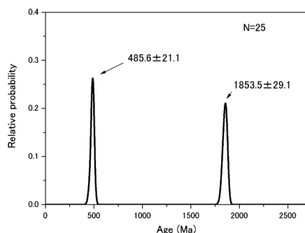
Fig. 2. Probability distribution of ages of detrital monazites from the sandstone, SD09, on Sado Island. Numerical value (n) denotes the number of analyzed monazite grains.
