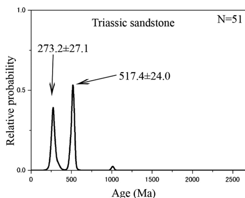
Fig. 2. Probability distribution of ages of detrital monazites from the sandstone, SD09, on Sado Island. Numerical value (n) denotes the number of analyzed monazite grains.
