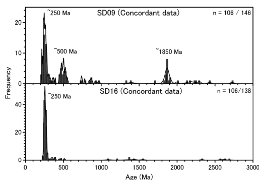
Fig. 3. Frequencies and probability distributions of concordant zircon ages from the samples, SD09 and SD16. Numerical value (n) denotes the number of analyzed zircon grains and concordant grains.
