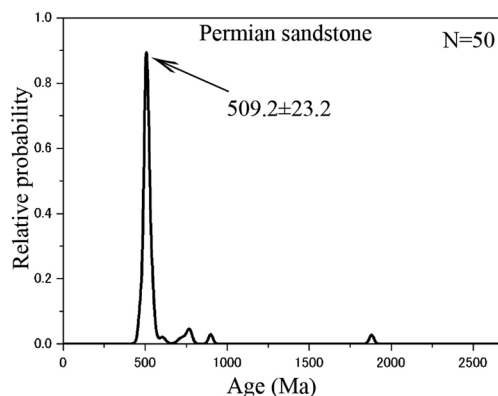
Fig. 4. Probability distribution of ages of detrital monazites from the Triassic and Permian sandstones from Vladivostok, south Primorye. Numerical value (n) denotes the number of analyzed monazite grains.
