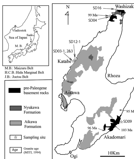
Fig. 1. Distribution of pre-Tertiary basement rocks on Sado Island and sampling sites for age analyses.
