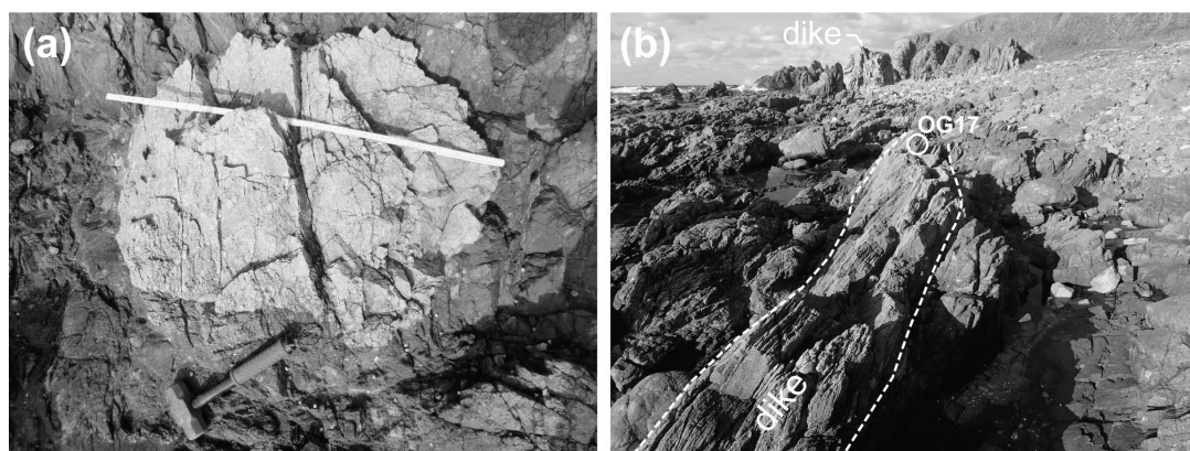
Fig. 2. Outcrop photos of the Akashima Formation. (a) Biotite granite xenolith (OG18) in the volcanic breccia of Akashima Formation. Scale = 80 cm. (b) Porphyritic rhyolite dike intruding into volcanic breccia. Thickness of the dike = ~60 cm. White circle corresponds to location where OG17 was sampled. Locations on the map is in Fig. 1 and coordinates are given in Table 1.
