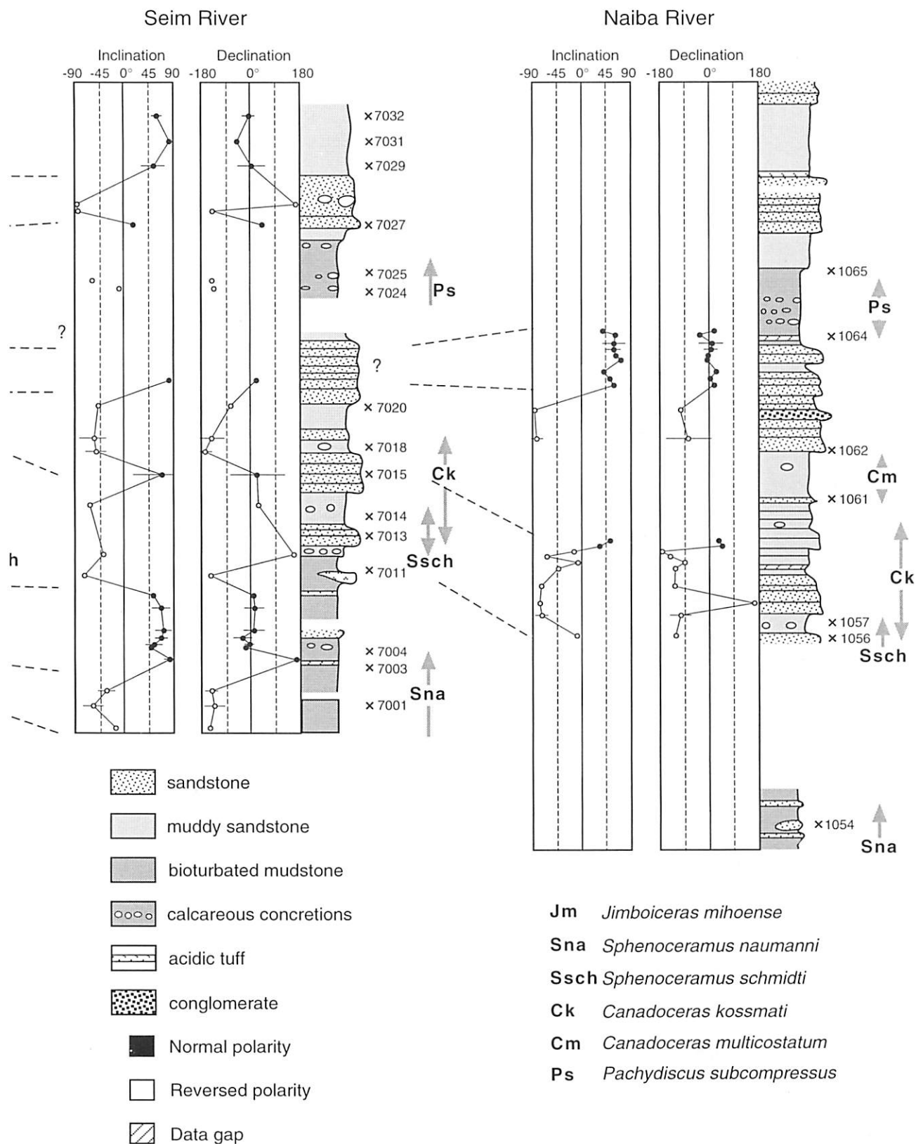
Figure 2. Lithology, magnetostratigraphy and ranges of selected zone fossils of the Krasnoyarka River, Seim River, and Naiba River sections. The boundaries between the magnetozone are placed at a midpoint between adjacent horizons of opposite magnetic polarity. Solid (open) circles show inclinations and declinations of normal (reversed) polarity, along with 95% confidence error bars if they can be computed from more than three individual sample directions. Broken lines indicate possible correlation of the magnetozone boundaries between sections.
