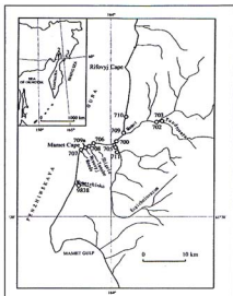
Fig. 1 Location of the Penzhinskaya Guba (Penzhina Gulf) area (1), Talovka River basin (2) and Pakhacha River basin (3) sequences. Localities: 9838 – Mametchinka River (lower Tyakryl Formation, Hauterivian); 707 – Mamet Cape (upper Karmalivayam Formation, Lower Aptian); 709a – Mysoviy Creek (lowermost Mamet Formation, Upper Albian?–Lower Cenomanian); 708 – Tanabe Creek (lower Mamet Formation, Lower Cenomanian); 706 – Shigeta Creek (upper Mamet Formation, Lower Cenomanian); 705 – Penzhinskaya Guba, 1 km W of the Eschichivayam River mouth (lower Penzhinskaya Formation, Upper Cenomanian); 711 – Eschichivayam River (left bank), 1.5 km upper of its mouth (middle Penzhinskaya Formation, lower Middle Turonian); 700 – Penzhinskaya Guba, 0.1–0.5 km NE of the Eschichivayam River mouth (middle Penzhinskaya Formation, middle Middle Turonian); 709 – Mamet River mouth (upper Bystrinskaya Formation, Upper Campanian); 710 – middle Penzhinskaya Formation (middle Middle Turonian); 702 – Mamet River, 5.5 km upper its mouth (lower Pilalvayam Formation, Upper Campanian); 703 – Tundrovaya River (middle Pilalvayam Formation, Lower Maastrichtian).
