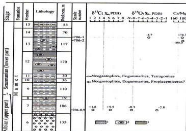
Fig. 5 The \delta^{18}\text{O} and \delta^{13}\text{C} values and Ca-Mg ratios of Lower Cenomanian bivalve calcite shells from the Penzhinskaya Guba. 1 - sandy siltstone, 2 - boulders, 3 - mudstone. Other designation as in Fig. 4.
