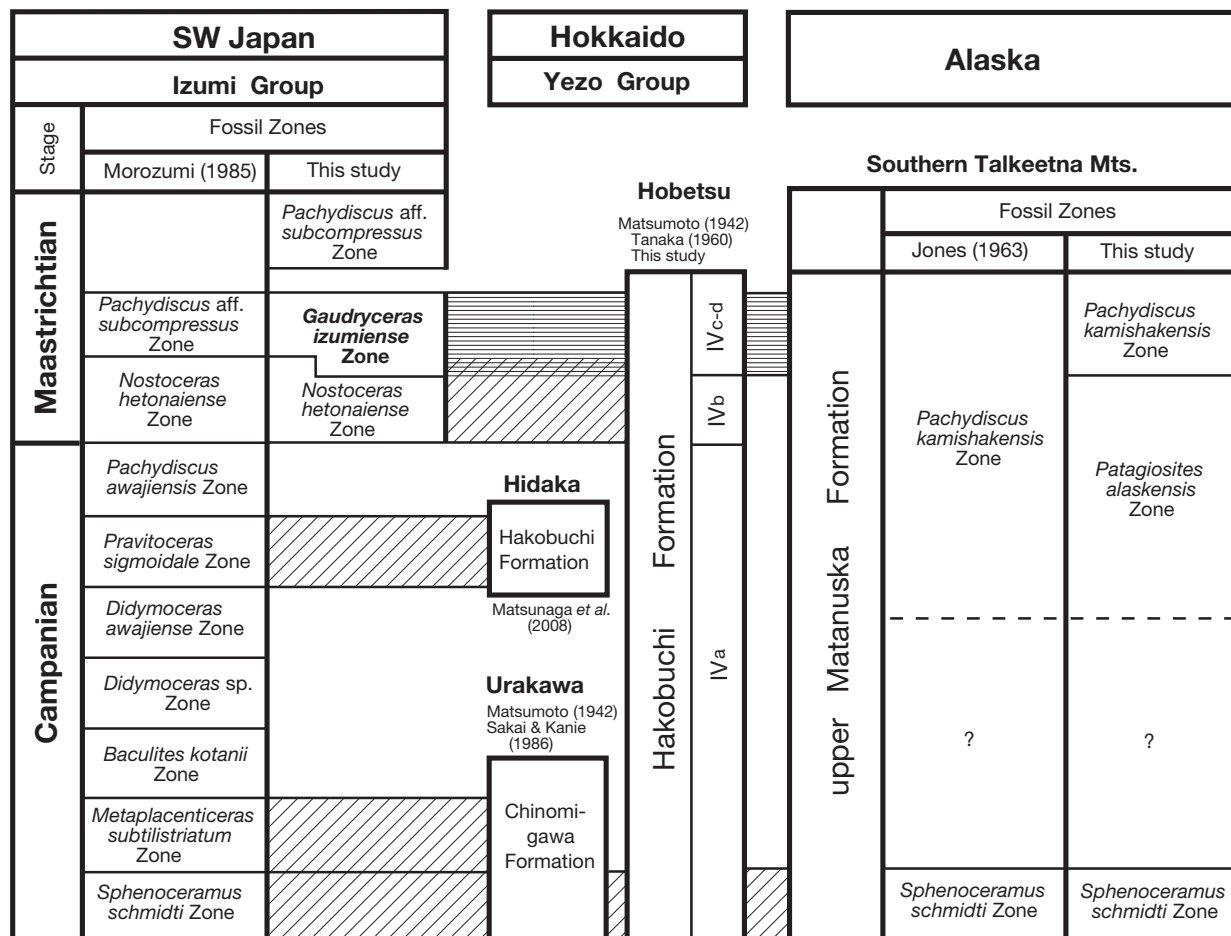
Figure 6. Diagram showing biostratigraphic correlation between Campanian-Maastrichtian deposits in Southwest Japan (left), Hokkaido (center) and Alaska (right). The lower Maastrichtian Gaudryceras izumiense Zone was first recognized in these three areas of the North Pacific realm.
