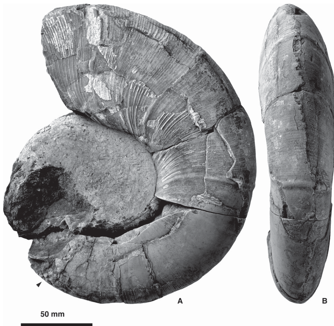
Figure 5. Gaudryceras izumiense Matsumoto and Morozumi, 1980, NSM PM23443, southern Talkeetna Mountains, Alaska. A. Right lateral view. Black arrow indicates position of last septum. B. Ventral view.
