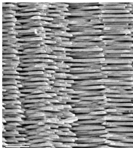
Fig. 2. Scanning electron micrograph of the ammonoid Grantzicerias affine (A-1), fragment of the shell whorl at H=51.0 mm showing microstructure of nacreous layer in cross-section, bar=3 \mu\text{m} ; lower Albian portion of the Matanuska Formation, Member 6; Ammonite Creek, southern Alaska.
