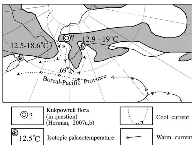
Fig. 5. Map showing palaeotemperatures determined on the basis of oxygen isotopic analysis (Zakharov et al., 2005 and original data), and some palaeofloristic data for the late part of the Early Albian (~107 Ma), Alaska–Koryak Upland area.
