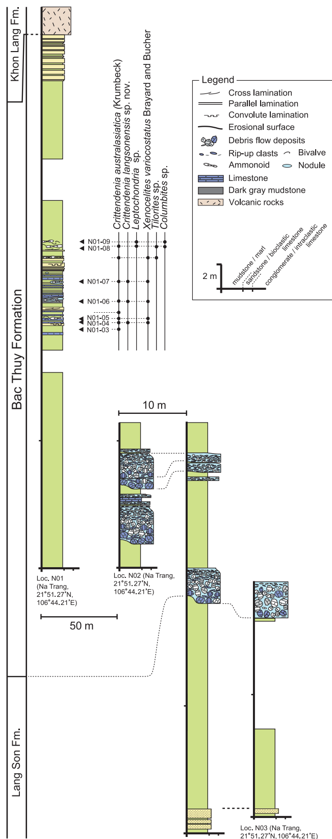
Figure 3. Columnar sections showing occurrence of molluscan fossils in Tung Huang and Na Trang villages, Lang Son City, northern Vietnam. Bivalves and ammonoids are abundantly found at Locs. N01–03–09. See Figure 1 for localities.
