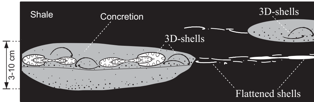
Figure 6. Schematic sketch of modes of fossil occurrence. Molluscan fossils are found abundantly in nodules and host shale. In the host shale, bivalves and ammonoids are completely flattened. Three-dimensional well preserved molluscs are obtained from calcareous nodules.
