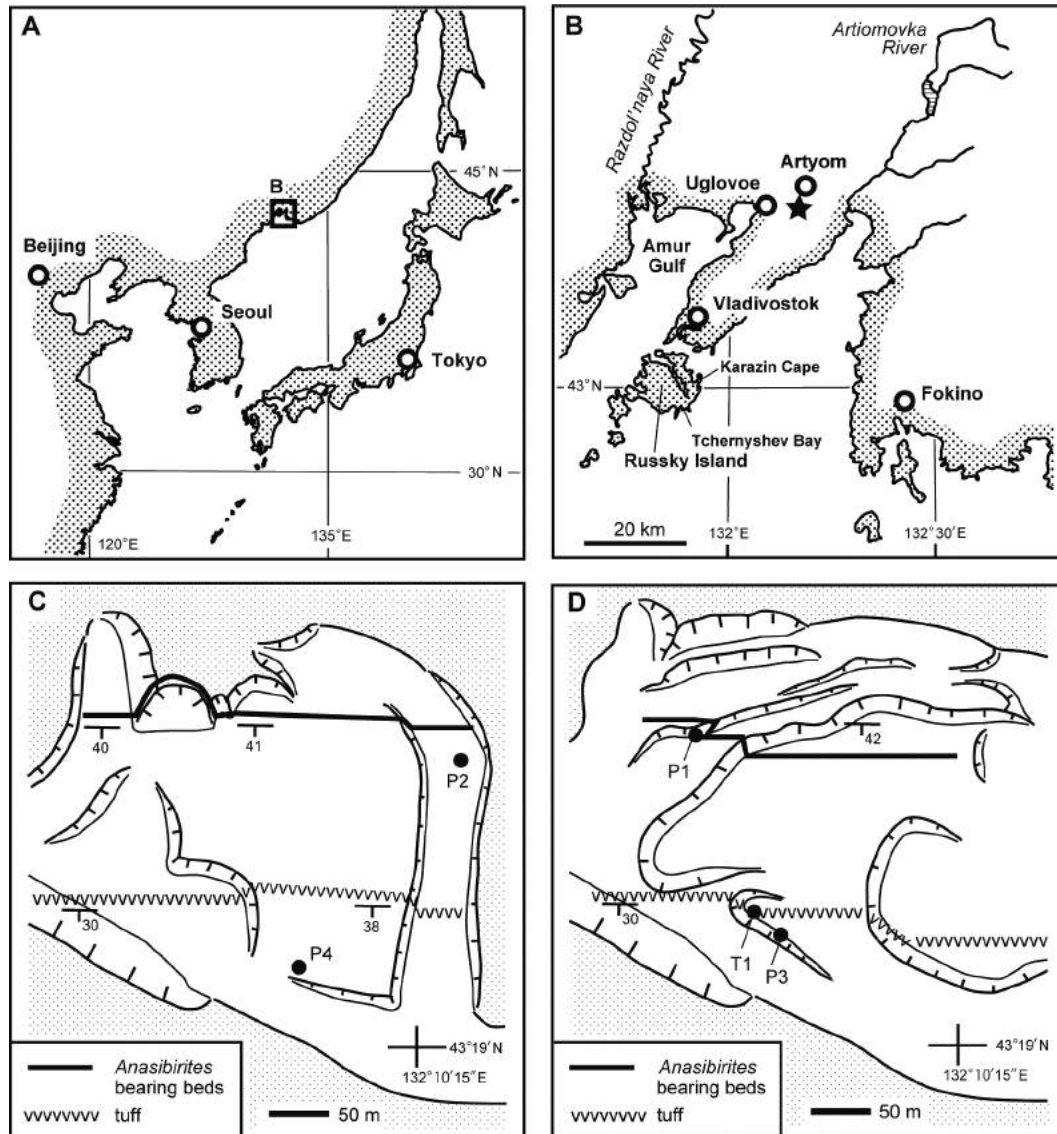
Figure 1. General map (A) showing location of South Primorye. Location (B) of the Artyom section indicated by star, and sketch maps (C, D) showing localities from which the Spathian ammonoids were collected. Quarry sketch maps C and D were made in 2005–2008 and 2011–2012 respectively. The 50–60-cm thick Anasibirites -bearing beds and the 30-cm thick white vitric tuff bed are widely traceable in the quarry.
