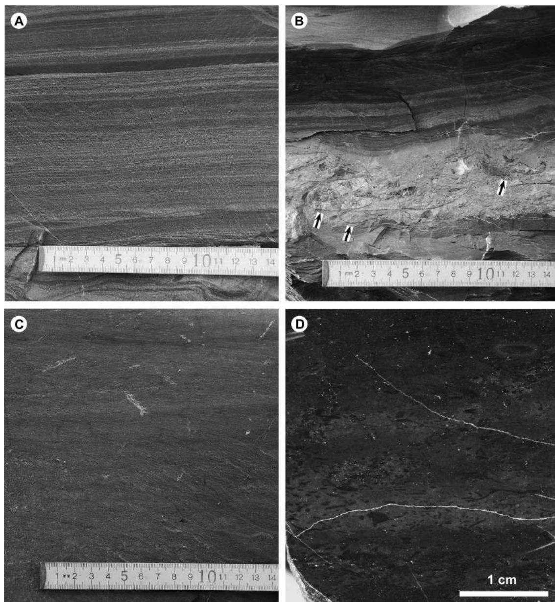
Figure 3. A, B, Mudstone with intercalations of fine-grained sandstone in the Smithian part of the Zhitkov Formation; A, Dark grey, well laminated mudstone; non-bioturbated lithology suggests a lack or near lack of benthic organisms under anoxic to dysoxic environment; B, fine-grained sandstone bed containing many ammonoids (arrows); ammonoid remains probably have been transported from their biotope to the deep basin by sediment gravity flow after death; C, D, mudstone in the Spathian part of the Zhitkov Formation; C, bioturbated, dark grey mudstone; D, vertical cross section of bioturbated mudstone; numerous mm-scale dark ovals which are small horizontal burrows of Phycosiphon isp., are concentrated at several levels.
