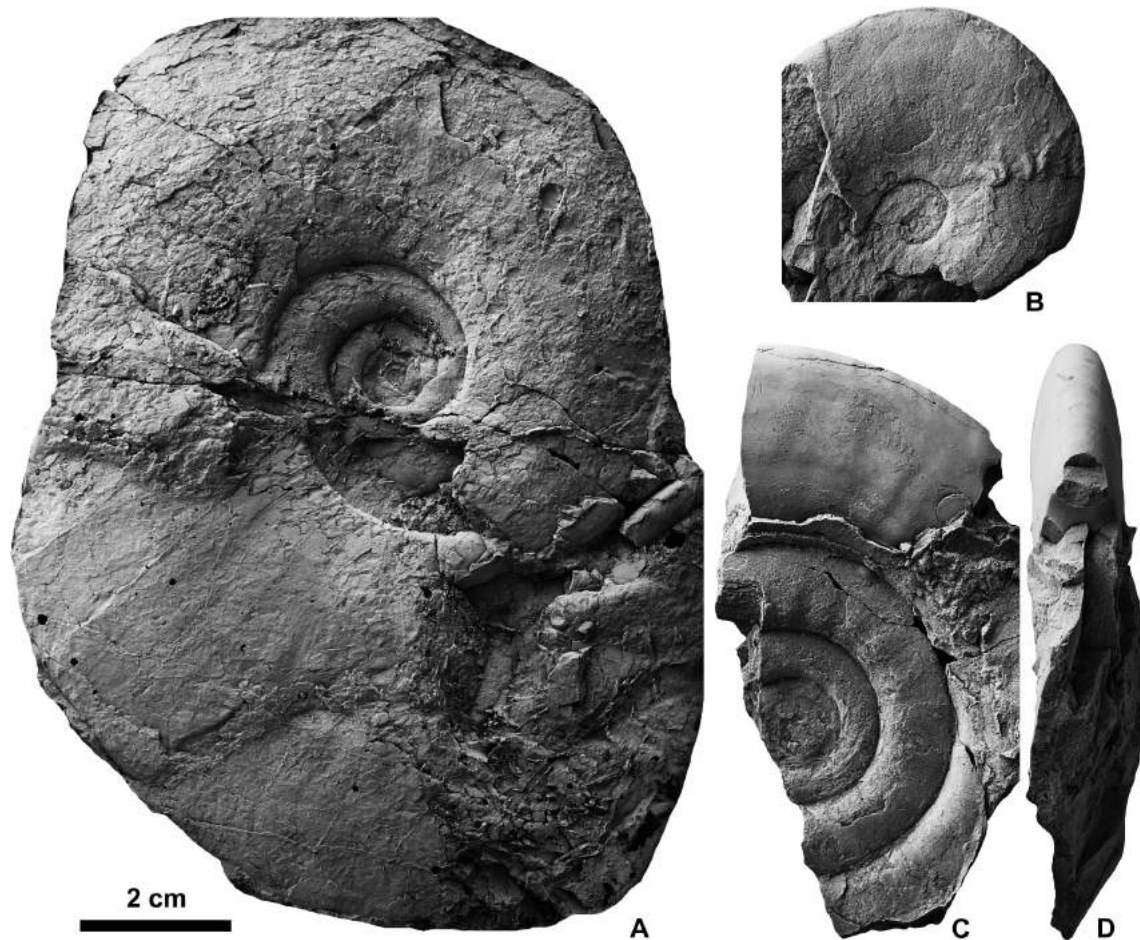
Figure 6. Ussuriphyllites and Leiophyllites from the Zhitkov Formation. A, B , Ussuriphyllites amurensis (Kiparisova, 1961); A, MNMS PM35055 (plastic cast of outer mold) from Loc. T1; right lateral view; B, MNMS PM35056 from Loc. P4; right lateral view; C, D , Leiophyllites sp., NMNS PM35059 from Loc. P4; C, right lateral view; D, ventral view.
