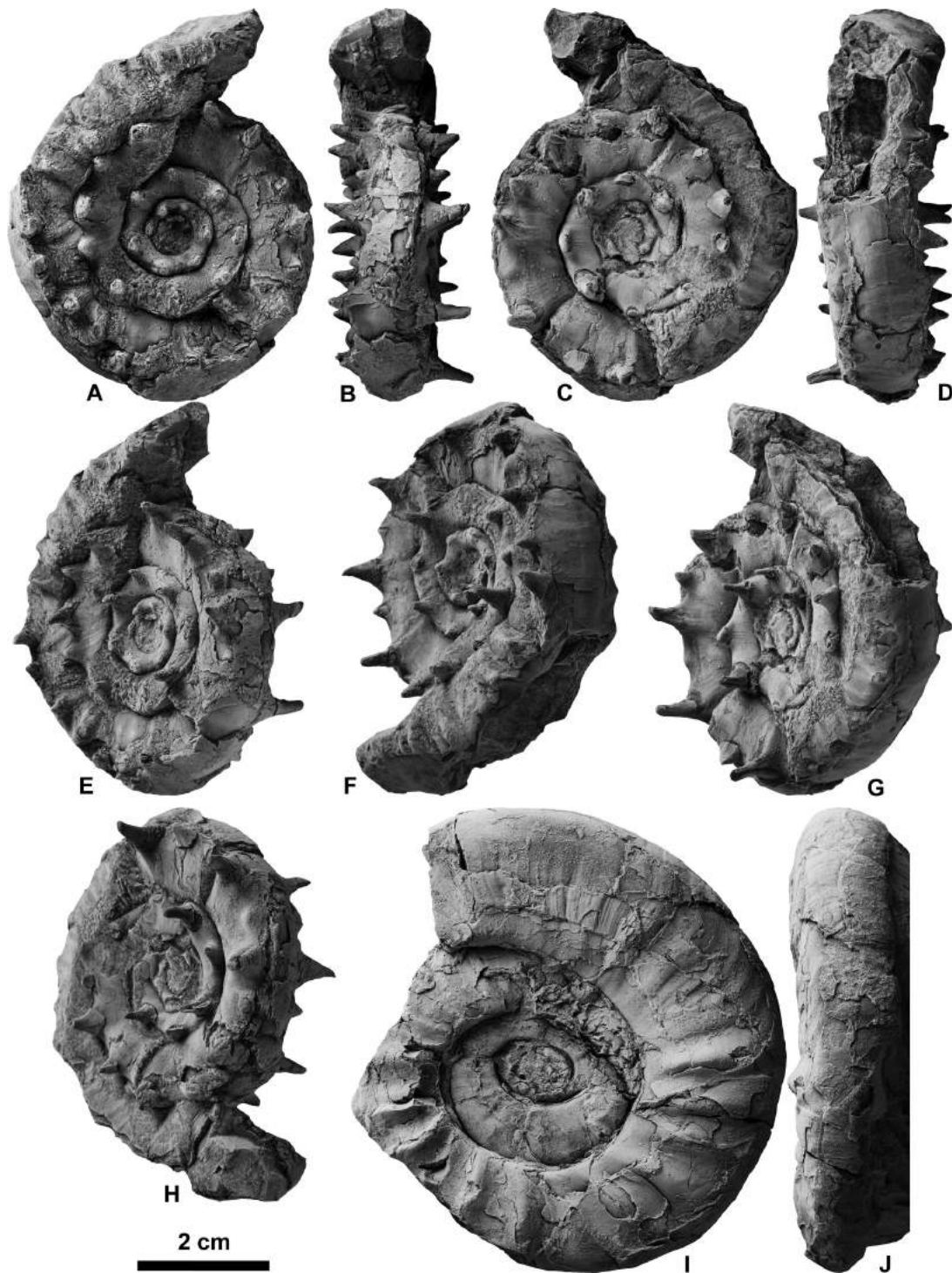
Figure 4. Tirolites and Bittnerites from the Zhitkov Formation. A–H , Tirolites longilobatus Shevyrev, 1968, NMNS PM35051 from Loc. P2; A, left lateral view; B, apertural view; C, right lateral view; D, ventral view; E, oblique apertural view, normal orientation; F, oblique ventral view, reversed orientation; G, oblique ventral view, normal orientation; H, oblique apertural view, reversed orientation; I, J , Bittnerites pacificus Zharnikova in Buryi and Zharnikova, 1981, NMNS PM35052 from Loc. P1; I, right lateral view; J, ventral view.
