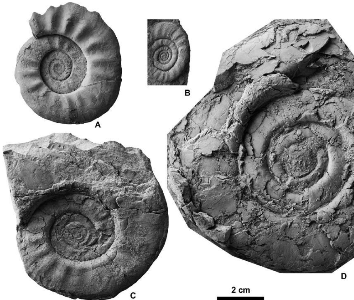
Figure 7. Leiophyllites sp. from the Zhitkov Formation. A , NMNS PM35060 from Loc. P4, right lateral view; B , NMNS PM35058 from Loc. P3, right lateral view; C , NMNS PM35061 from Loc. P4, right lateral view; D , NMNS PM35057 (plastic cast of outer mold) from Loc. P3, left lateral view.
