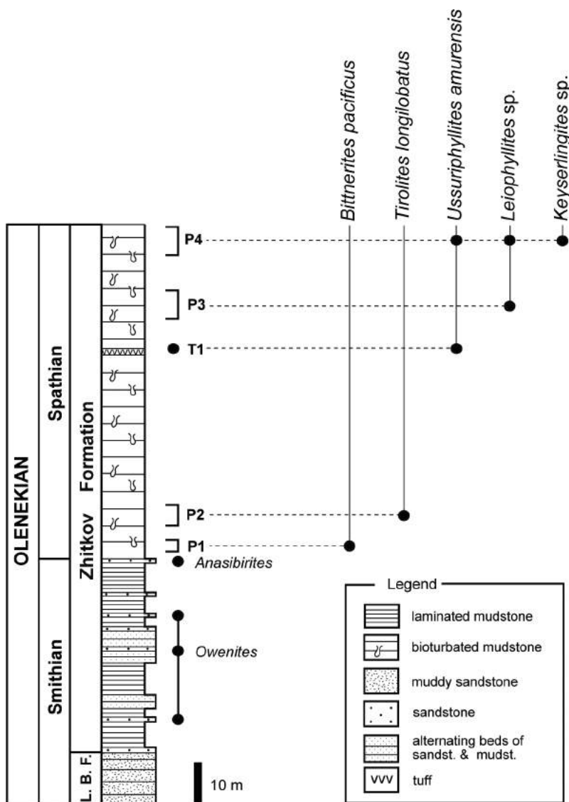
Figure 2. Lithology and stratigraphic occurrence of ammonoids in the Lower Triassic Artyom section. L.B.F.: Lazurnaya Bay Formation.
