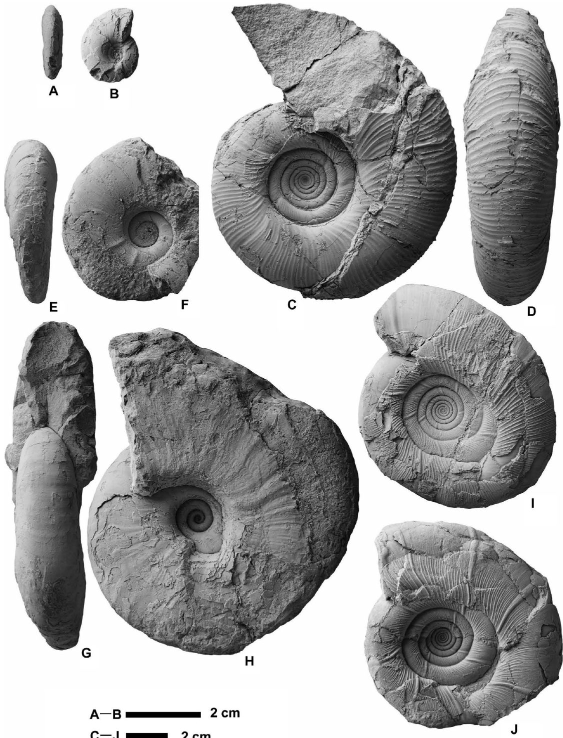
Fig. 3. Important ammonoids from the Heitaro-zawa Formation along the Nakanokawa River. A, B, Zalandites varuna , NMNS PM35456, from loc. 1036; C, D, Gaudryceras makarovense , NMNS PM35457, from a float concretion found at loc. 2032; E–H, Pachydiscus flexuosus ; E, F, NMNS PM35458, from loc. 2033 (collected by Y. Tsujino); G, H, NMNS PM35459, from loc. 2034; I, Gaudryceras sp., NMNS PM35460, from a float concretion found at loc. 2035; J, Gaudryceras hamanakense , NMNS PM35461, from loc. 2037.
