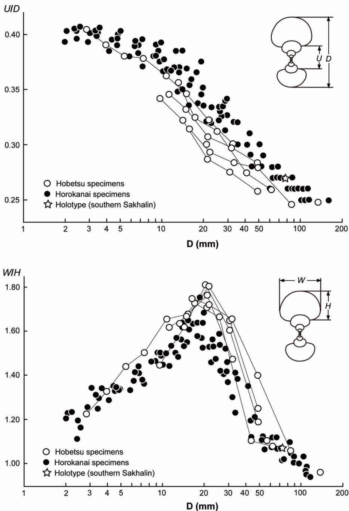
Figure 8. Scatter diagrams showing ontogenetic variation in umbilical diameter/shell diameter ( U/D ) versus shell diameter ( D ) and whorl width/whorl height ( W/H ) versus shell diameter for Parajaubertella kawakitana Matsumoto, 1943 from the Hobetsu (white circles) and Horokanai (black circles) areas and the holotype UMUT MM 19698 from southern Sakhalin (white star), based on data from Shigeta et al. (2023).
