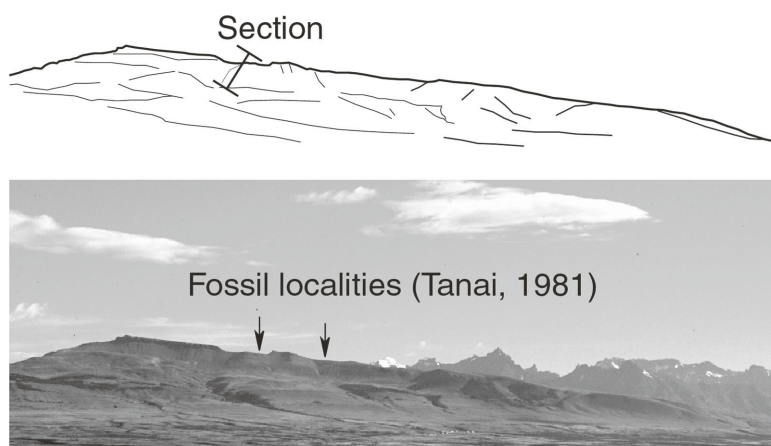
Fig. 2. Overview of Cerro Guido, showing localities of plant megafossils reported by Tanai (1981) and stratigraphic section for this study.
