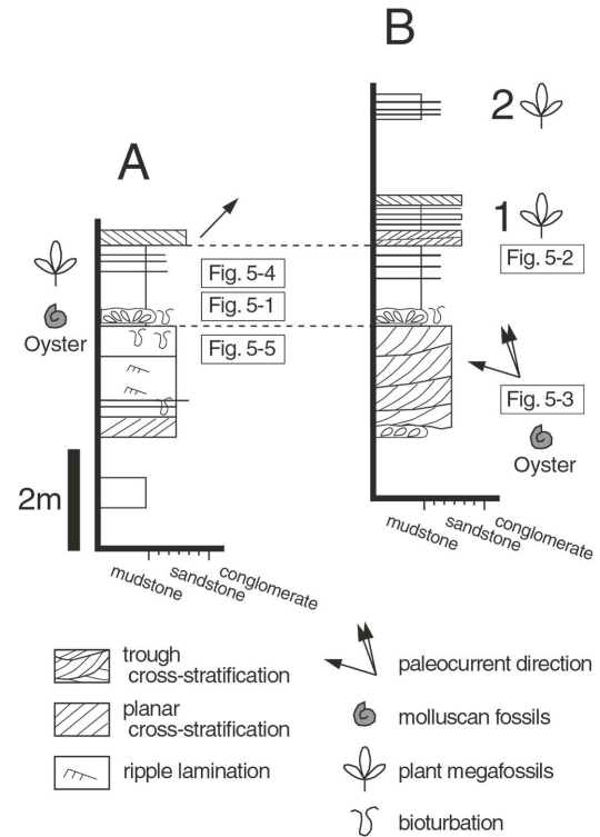
Fig. 4. Detailed columnar sections around the plant megafossil localities of the Dorotea Formation. Section A locates approximately 10 m west of section B.
