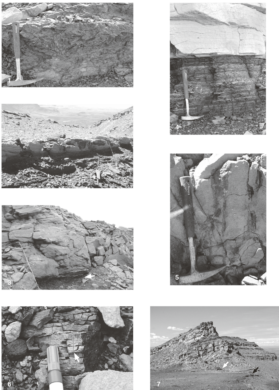
Fig. 5. 1, Close-up view of the upper oyster bed; 2, Plant megafossil locality 1; 3, Sandstone between two oyster beds, which is characterized by trough cross-stratification. Arrow represents lower oyster bed shown in Fig.4B. Scale equals 1 m; 4, Lagoonal facies represented by thinly laminated mudstone and sandstone; 5, Vertical, cylindrical burrow found in unit 7. Just below the upper oyster bed at Fig. 3A; 6, Root trace at unit 8 (arrow). A pen cap for scale is 2.8 cm long; 7, Overview of the upper part of the Dorotea Formation, east of plant megafossil localities 1 and 2. Solid arrow indicates upper oyster bed, and an open arrow represents plant-bearing beds. Hammer for scale has a handle 30 cm long (Figs. 5-1, 2, 4, and 5).
