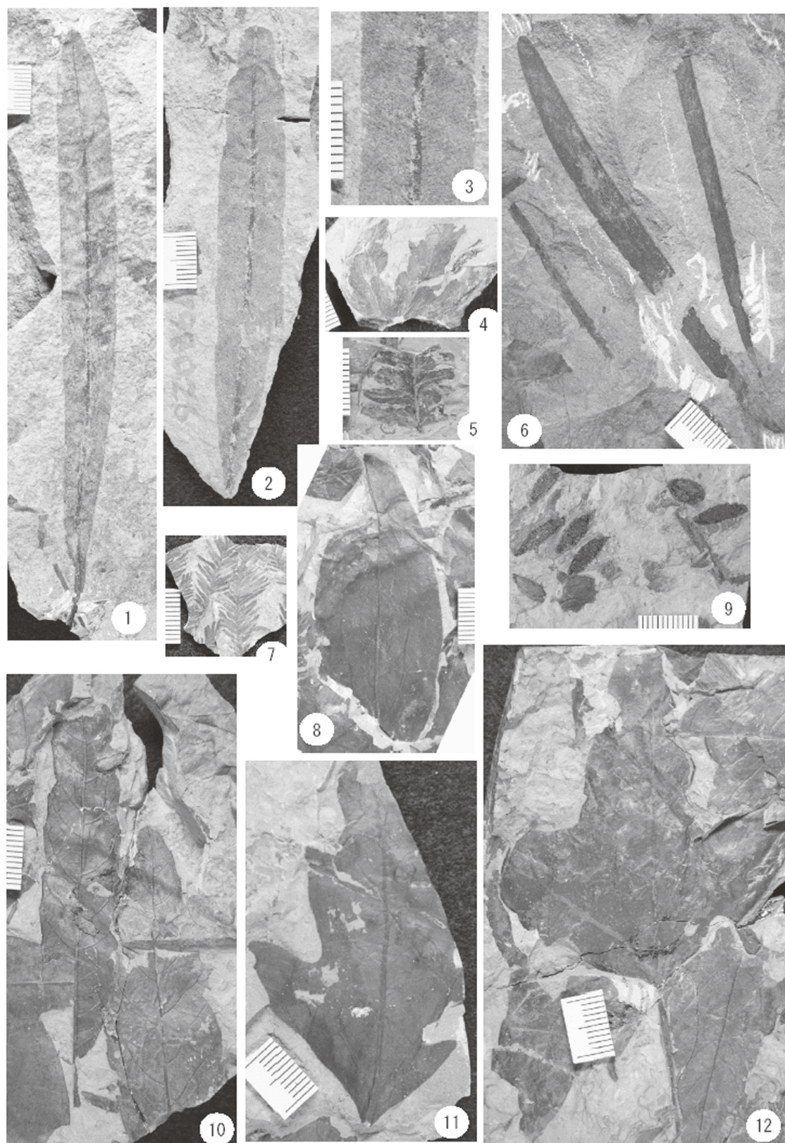
Fig. 6. Selected plant megafossils from the Dorotea Formation at Cerro Guido.
