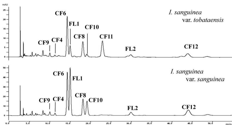
Fig. 14. HPLC comparisons of C-glycosylflavones and flavonols from the leaves of Iris sanguinea var. sanguinea and var. tobataensis . CF4 = swertiajaponin, CF6 = swertisin 2''-O-glucoside (flavoayamenin), CF8 = swertisin, CF9 = isoorientin 2''-O-glucoside, CF10 , 11 = acetylated swertisin 2''-O-glucosides, CF12 = acetylated swertisin, FL1 = myricetin 3-O-rhamnoside, and FL2 = quercetin 3-O-rhamnoside. Wave-length is 340 nm.
