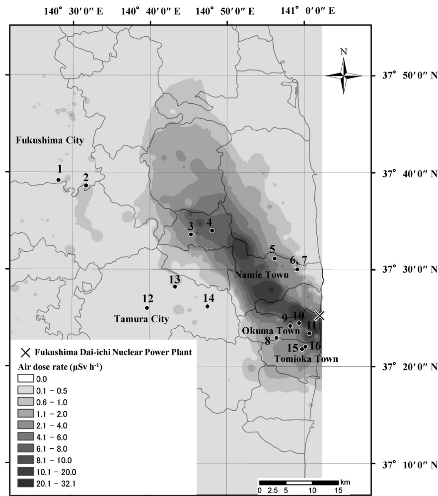
Fig. 1. Locations of lichen sampling points superimposed on an air dose rate map measured by MEXT in June and July 2011 (MEXT, 2011a and 2011b).
