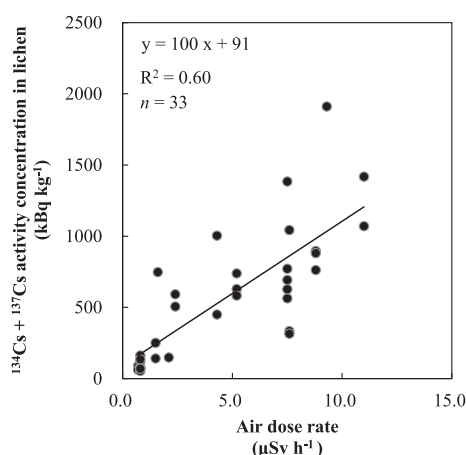
Fig. 4. The relationship between ^{134}\text{Cs} + ^{137}\text{Cs} activity concentration in lichen and the air dose rate at sampling points (without snow cover). The radiocaesium activity concentration in lichen was decay corrected to the date of each lichen sampling. Air dose rate was measured at each lichen sampling date. The regression equation was calculated by simple linear regression analysis ( P < 0.001 ). The slope and intercept values of the regression line were 100 \pm 30 and 91 \pm 180 , respectively (95% confidence interval). The Spearman's rank correlation coefficient was calculated as 0.84 ( P < 0.01 ).
