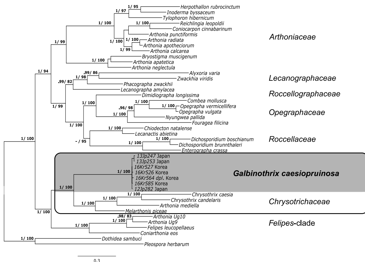
Figure 2. Bayesian 50% majority-rule consensus tree showing the position of Galbinothrix caesiopruinosa at the base of Chrysotrichaceae in Arthoniales . Support values from the Bayesian (first) and the RAxML (second) analysis are indicated on the branch nodes.
