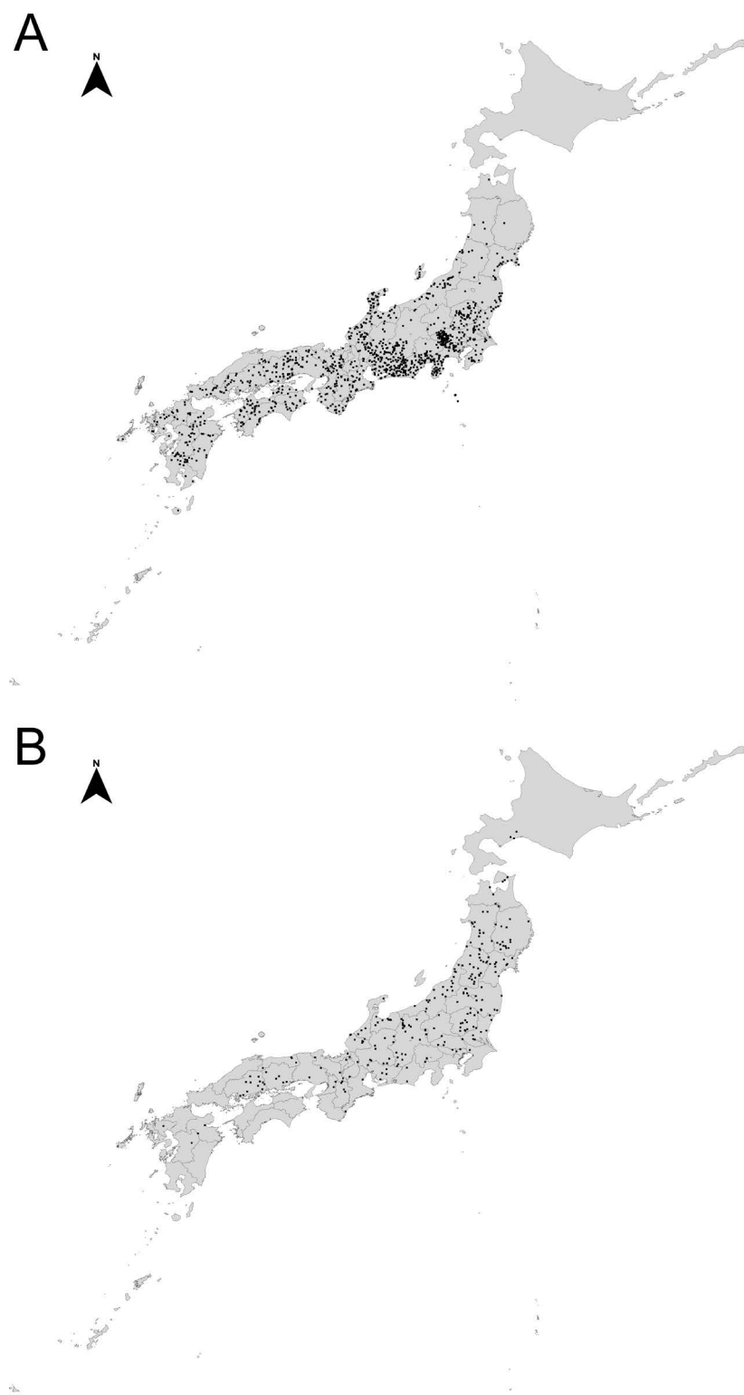
Fig. 3. Distribution maps of the Thelypteris japonica complex in Japan based on the specimens examined by the present study. A. Thelypteris japonica forma japonica ; B. T. japonica forma formosa .
