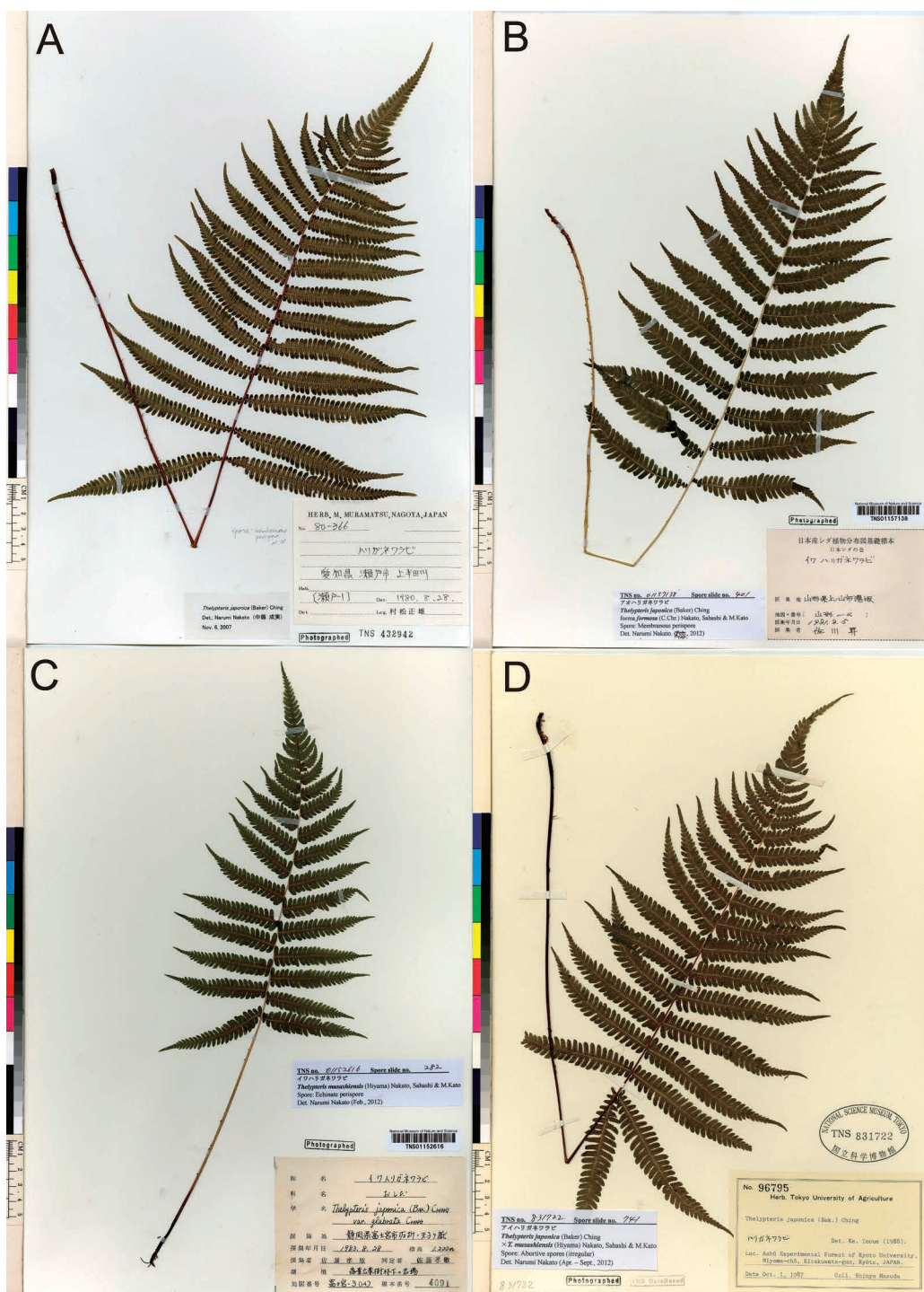
Fig. 1. Specimens of the Thelypteris japonica complex in Japan. A. Thelypteris japonica forma japonica (TNS-VS-432942, Aichi Pref., Seto-shi, M. Muramatsu 80366); B. T. japonica forma formosa (TNS-VS-1157138, Yamagata Pref., Kaminoyama-shi, N. Sagawa s.n.); C. T. musashiensis (TNS-VS-1152616, Shizuoka Pref., Fujinomiya-shi, T. Sato 4091); D. T. japonica × T. musashiensis , the castaneous stipe form (TNS-VS-831722, Kyoto Pref., Kitakuwada-gun, Miyama-cho, S. Masuda s.n.).
