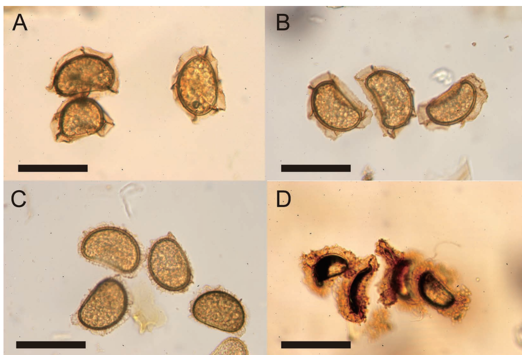
Fig. 2. Spores of the Thelypteris japonica complex in Japan (scale bars = 50 µm). A. spores with membraneous ornamentation produced by T. japonica forma japonica (TNS-VS-397231, Yamaguchi Pref., Iwakuni-shi, A. Minami 16677); B. spores with membraneous ornamentation produced by T. japonica forma formosa (TNS-VS-438920, Fukushima Pref., Onuma-gun, Showa-mura, Z. Kaneda s.n.); C. spores with echinate ornamentation produced by T. musashiensis (TNS-VS-1159828, Oita Pref., Naoiri-gun, Kuju-machi, M. Arakane s.n.); D. irregular-shaped spores of T. japonica × T. musashiensis (TNS-VS-438936, Fukushima Pref., Kitakata-shi, Z. Kaneda 6517).
