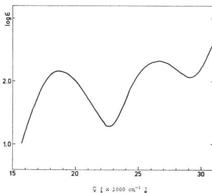
Fig. 5. The absorption spectrum of the complex ion (\pm)\text{-}[Co(ox)(2,2'\text{-bip})_2]^+ in H_2O .
