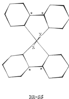
Fig. 4. The meso structure of the trans -diacido complexes. X shows the nitro or the chloro group.
