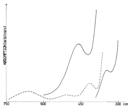
Fig. 1. The absorption spectra of (\pm)\text{-trans-}[\text{Co}(\text{NO}_2)_2(2,2'\text{-bip})_2]^+ in \text{H}_2\text{O} and (\pm)\text{-trans-}[\text{CoCl}_2(2,2'\text{-bip})_2]^+ in \text{CH}_3\text{OH} . The broken line indicates the latter complex ion.
