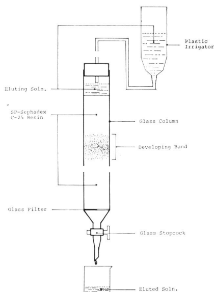
Fig. 8. The brief illustration of the column-chromatographic apparatus.
