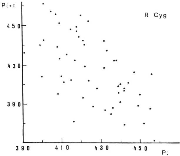
Fig. 7. First return map of R Cyg.
