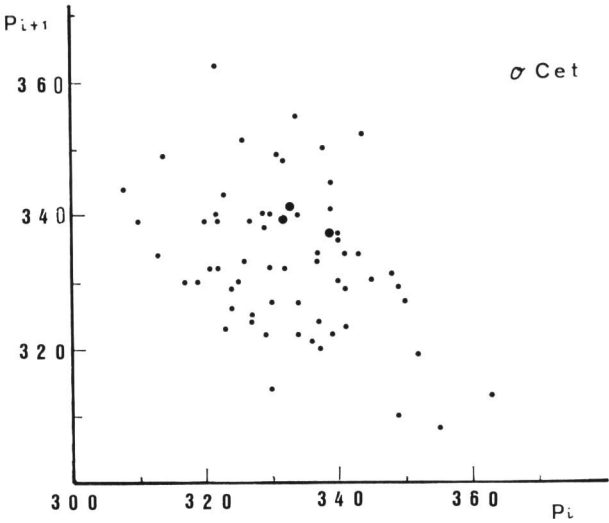
Fig. 6. First return map of \sigma Cet.
