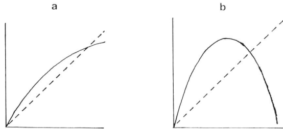
Fig. 1. Schematic first return maps. The horizontal axis indicate T(i) and the vertical axis T(i+1) .
