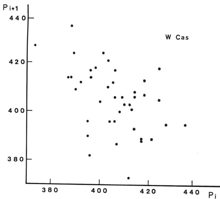
Fig. 5. First-return map of W Cas.
