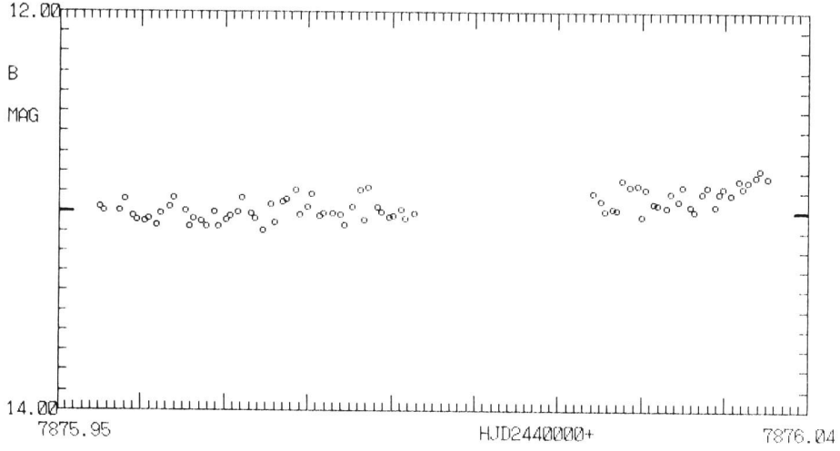
Figure 2. Light curve in B
