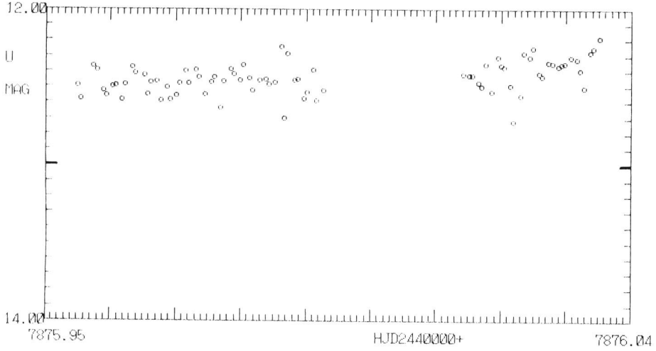
Figure 3. Light curve in U
