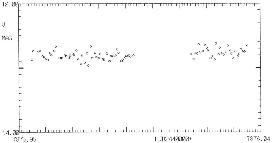
Figure 1. Light curve in V
