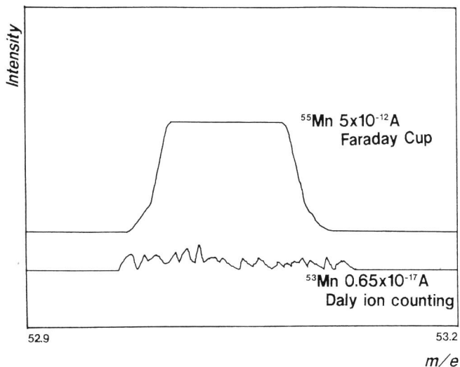
Fig. 3. An example of the mass-scan in the range 52.9–53.2 at the Daly detector position. At the Faraday detector position, it corresponds to 54.9–55.2. The full range of the intensity are 10^{-11} A and 10^{-16} A for ^{55}\text{Mn} and ^{53}\text{Mn} , respectively.
