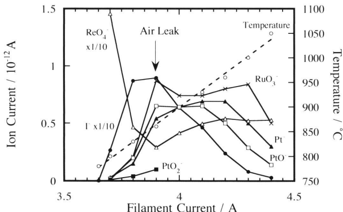
Fig. 1. The observed negative thermal ion currents from a Br, I, Ru and Re mixed calibration solution against filament currents. The measured mass numbers for \text{I}^- , \text{RuO}_3^- , \text{Pt}^- , \text{PtO}^- , \text{PtO}_2^- and \text{ReO}_4^- were 127, 150, 194, 210, 226 and 251, respectively. Filament temperatures measured by an optical pyrometer are also shown.
