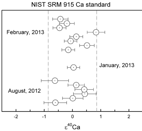
Fig. 2. Results of 15 replicate runs of isotopic ratio measurements on the Ca standard (NIST SRM 915a) using Faraday cups. \varepsilon^{40}\text{Ca} = [({}^{40}\text{Ca}/{}^{44}\text{Ca})_{\text{each value}}/47.1641 - 1] \times 10^4 , where 47.1641 is an average value of {}^{40}\text{Ca}/{}^{44}\text{Ca} ratio for SRM 915a standard ( 2\text{SD} = \pm 0.0040 , n = 15 ). Error bars are 2 sigma standard errors.
