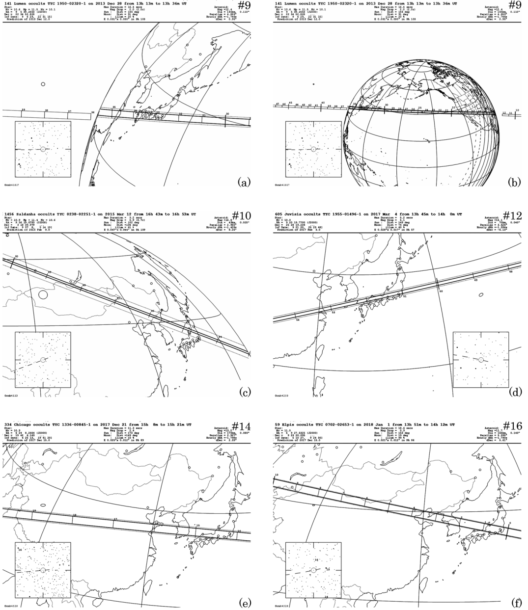
Fig. 3. Maps of predicted path of asteroidal occultation 3) . The larger the size of an asteroid is, the wider the strip in which the occultation can be observed is. The insets are star charts that show how the asteroid approaches to the occulted star. The number at the upper right of each figure corresponds to the serial number of occultation in Table 1, i.e., Fig. 3a is of the occultation #9 by the asteroid (141) Lumen, for example. Fig. 3b shows that the occultation by (141) Lumen can be observed also at the west coast of the U.S.A.
