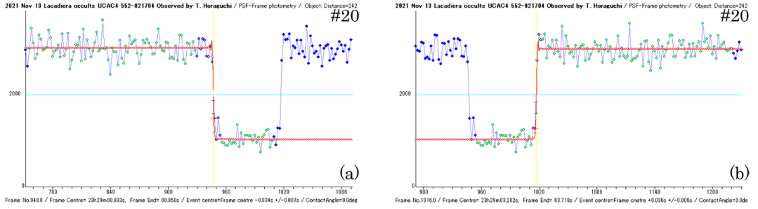
Fig. 2. Light curves of the occultation #20 by the asteroid (336)Lacadiëra. The horizontal axes are video frame number, and the vertical axes are brightness. The respective red line shows the result of fitting to determine the time of (a) disappearance and (b) reappearance by Limovie (8,9) .
