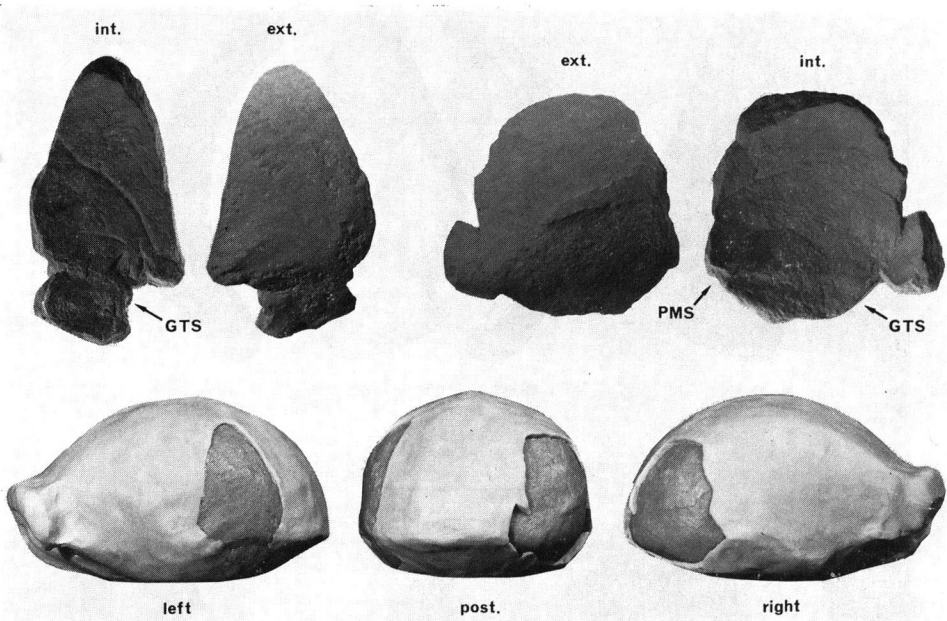
Fig. 3. Plaster casts of the S 37a left P-M-O fragment (left) and S 37b right P-O fragment (right), and reconstructed skull vault showing the positions of the fragments. Details of the surface structure are seen in the casts. GTS, groove for the transverse sinus; PMS, parietomastoid suture.
